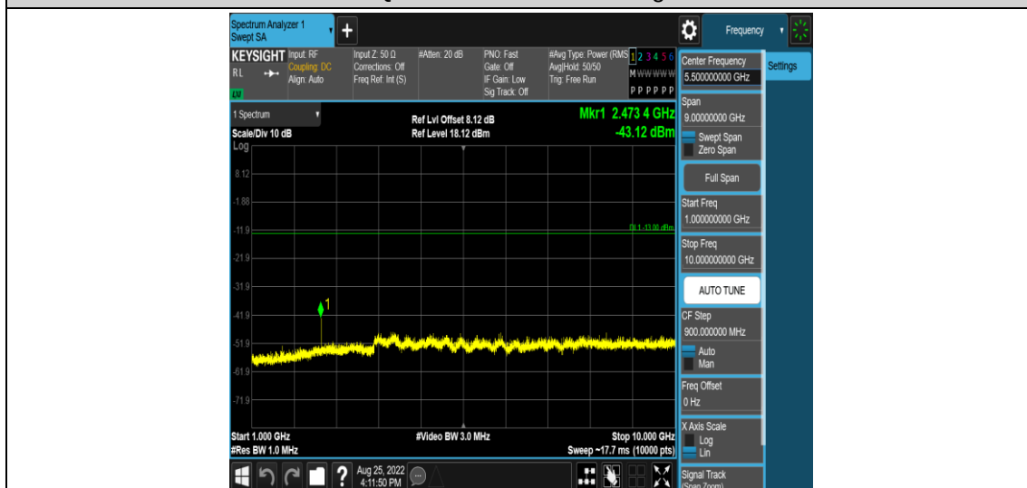
Band26-10MHz-QPSK-26840-1RB#0-Range4:1000~10000MHz
