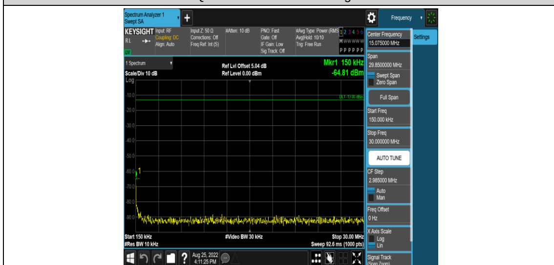
Band26-10MHz-QPSK-26840-1RB#0-Range2:0.15~30MHz
