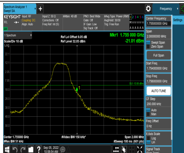
Band4-3MHz-QPSK-20385-1RB#14
