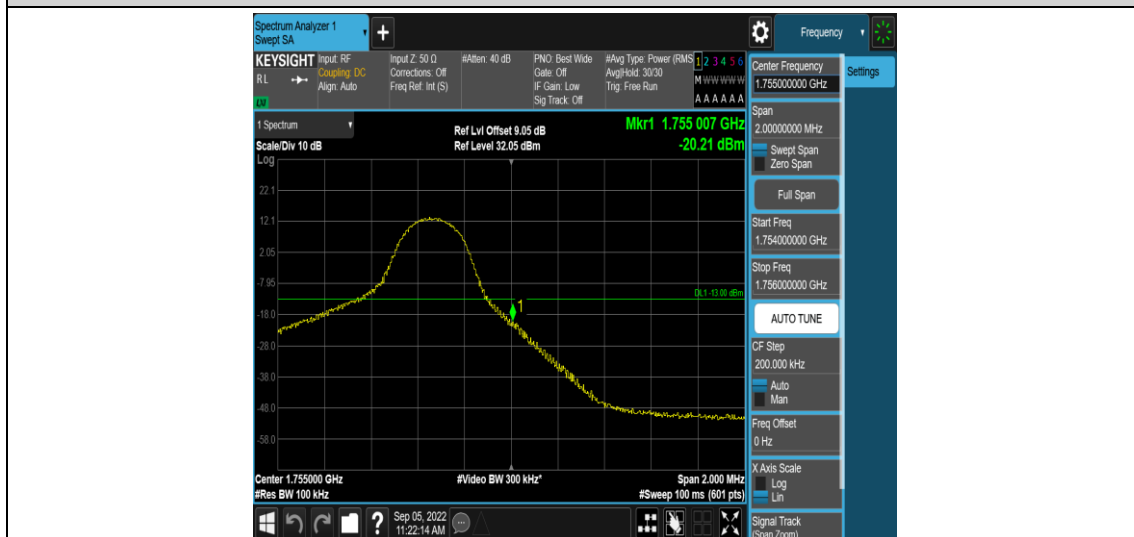
Band4-5MHz-16QAM-20375-1RB#24
