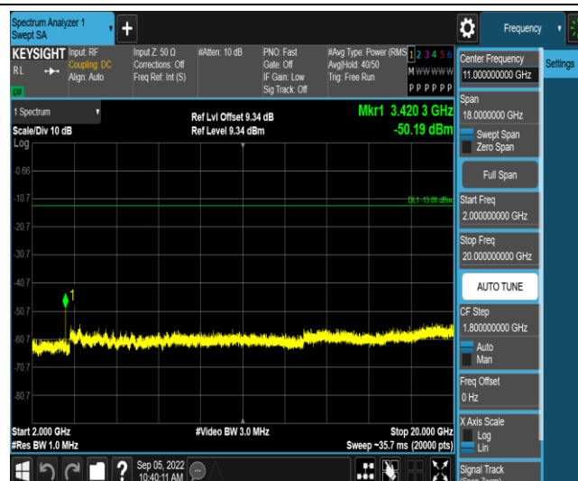
Band4-1.4MHz-QPSK-19957-1RB#0-Range5:2000~20000MHz
