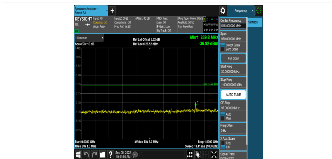
Band4-1.4MHz-QPSK-20175-1RB#0-Range3:30~1000MHz
