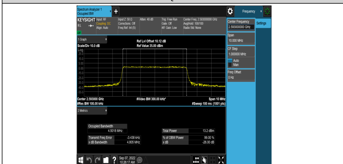
Band41-5MHz-16QAM-40620-25RB#0
