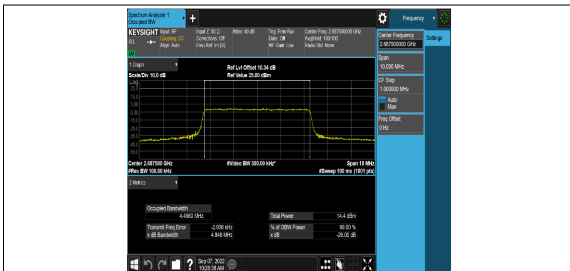
Band41-5MHz-QPSK-41565-25RB#0
