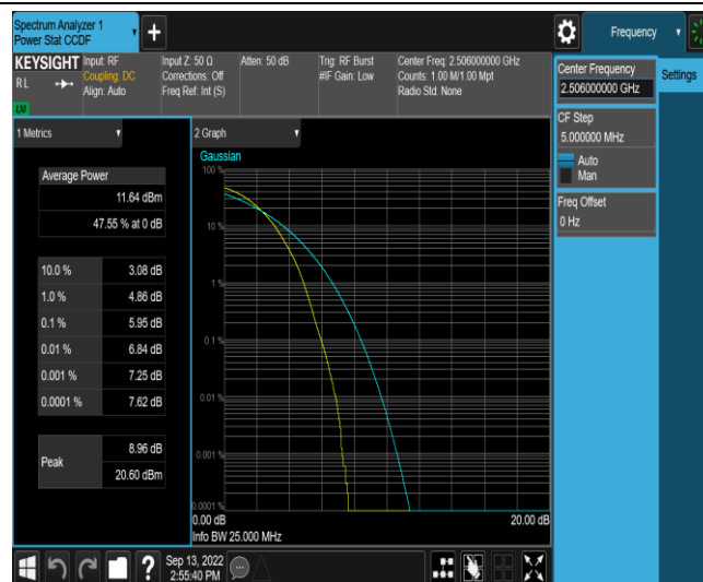
Band41-20MHz-16QAM-39750-1RB#0
