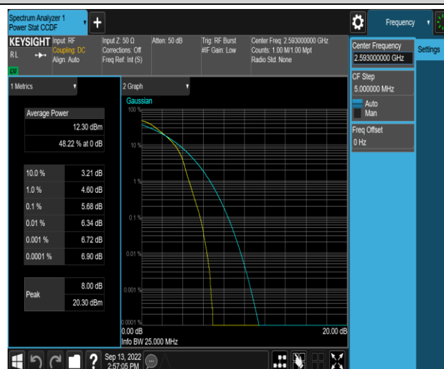
Band41-20MHz-16QAM-40620-1RB#0
