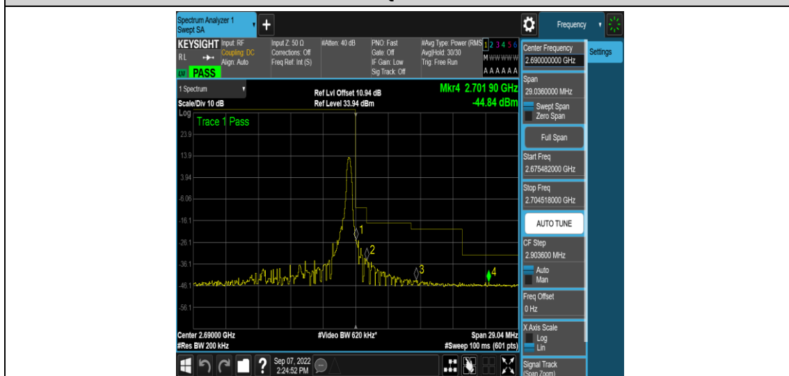
Band41-10MHz-QPSK-41540-1RB#49
