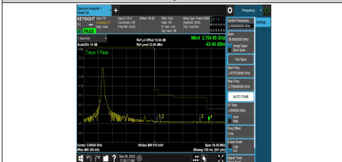
Band41-15MHz-16QAM-41515-1RB#0
