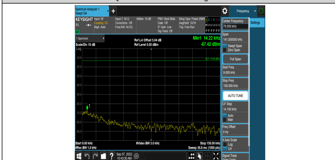
Band41-5MHz-QPSK-41565-1RB#0-Range1:0.009~0.15MHz
