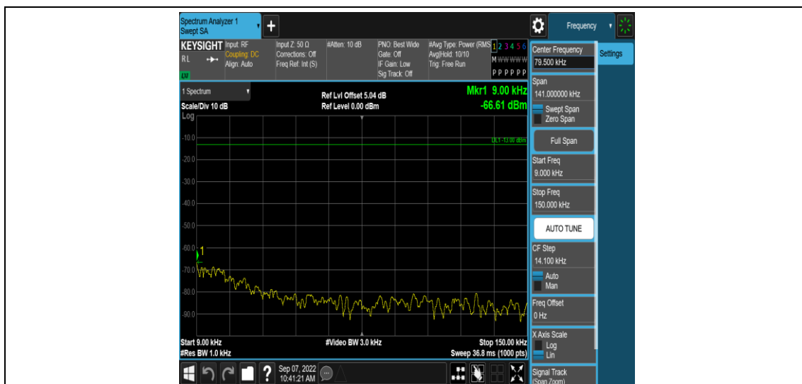
Band41-5MHz-QPSK-40620-1RB#0-Range1:0.009~0.15MHz
