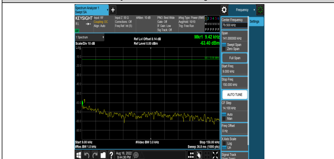
Band5-3MHz-16QAM-20635-1RB#0-Range1:0.009~0.15MHz
