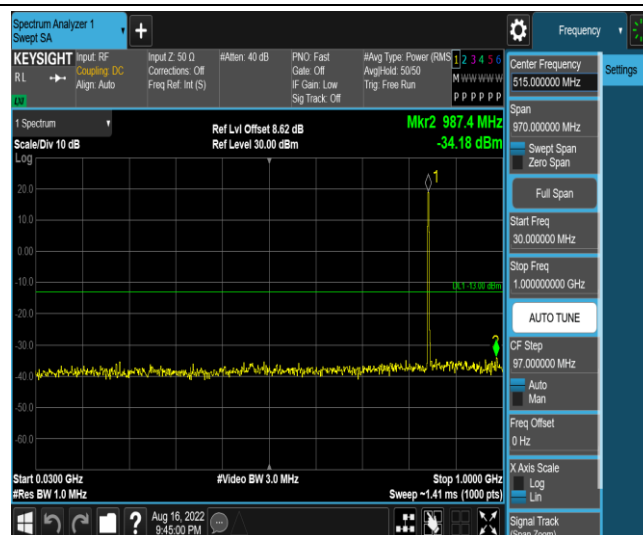
Band5-3MHz-16QAM-20635-1RB#0-Range3:30~1000MHz
