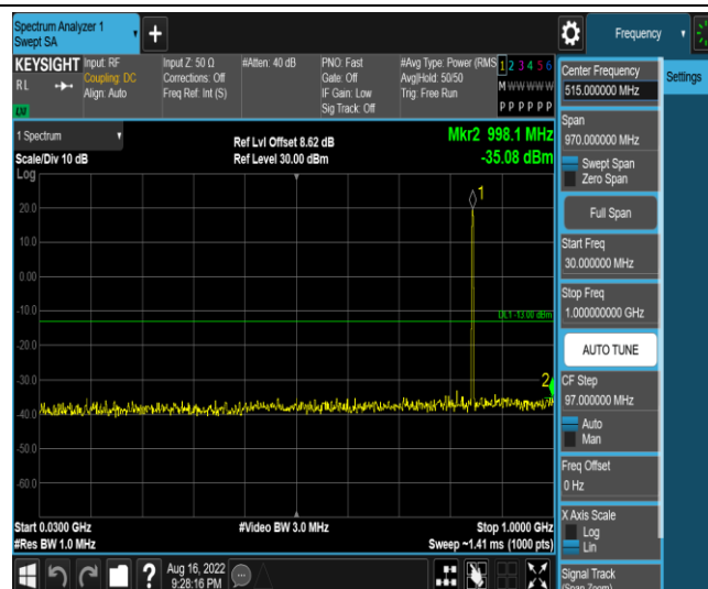
Band5-1.4MHz-QPSK-20643-1RB#0-Range3:30~1000MHz
