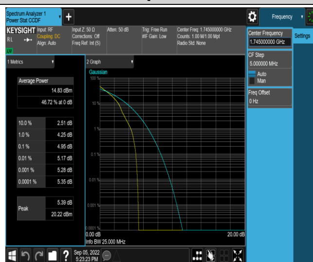
Band66-15MHz-QPSK-132322-1RB#0
