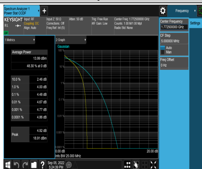
Band66-15MHz-QPSK-132597-75RB#0
