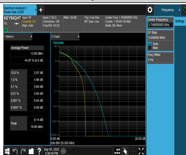
Band66-3MHz-16QAM-132322-1RB#0
