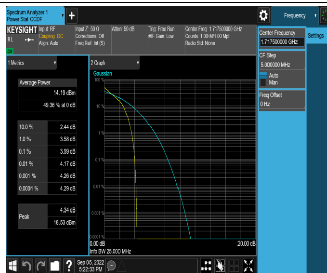
Band66-15MHz-QPSK-132047-1RB#0
