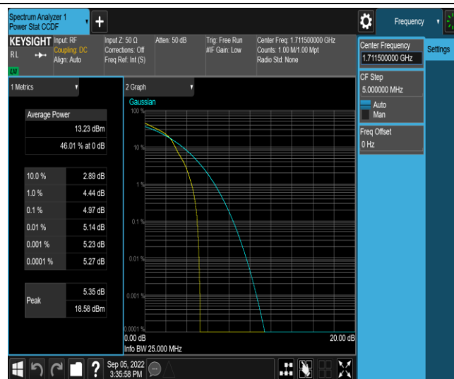
Band66-3MHz-16QAM-131987-1RB#0
