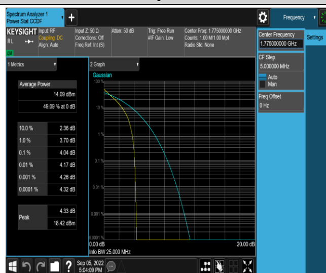
Band66-10MHz-QPSK-132622-50RB#0
