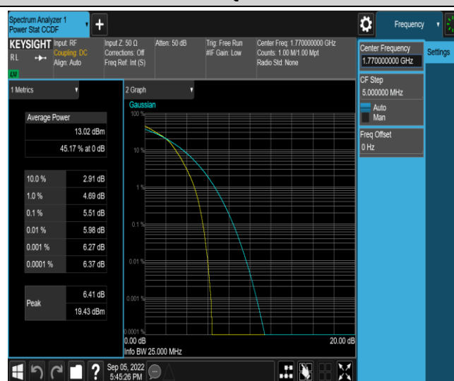
Band66-20MHz-16QAM-132572-100RB#0
