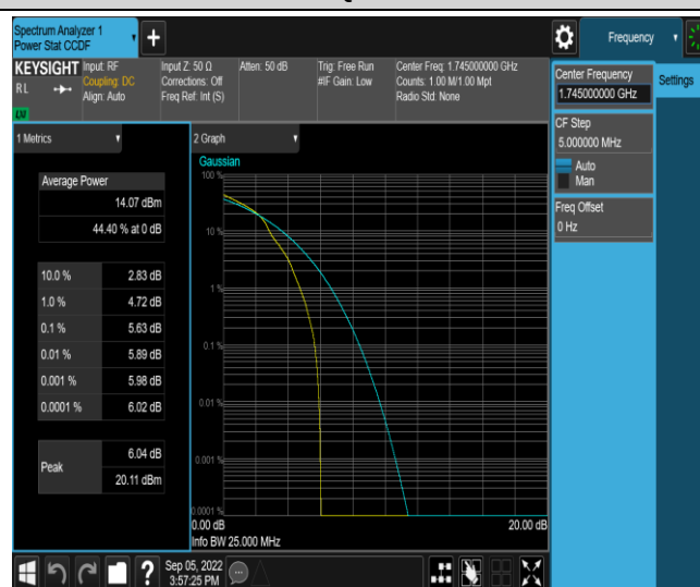
Band66-5MHz-16QAM-132322-1RB#0
