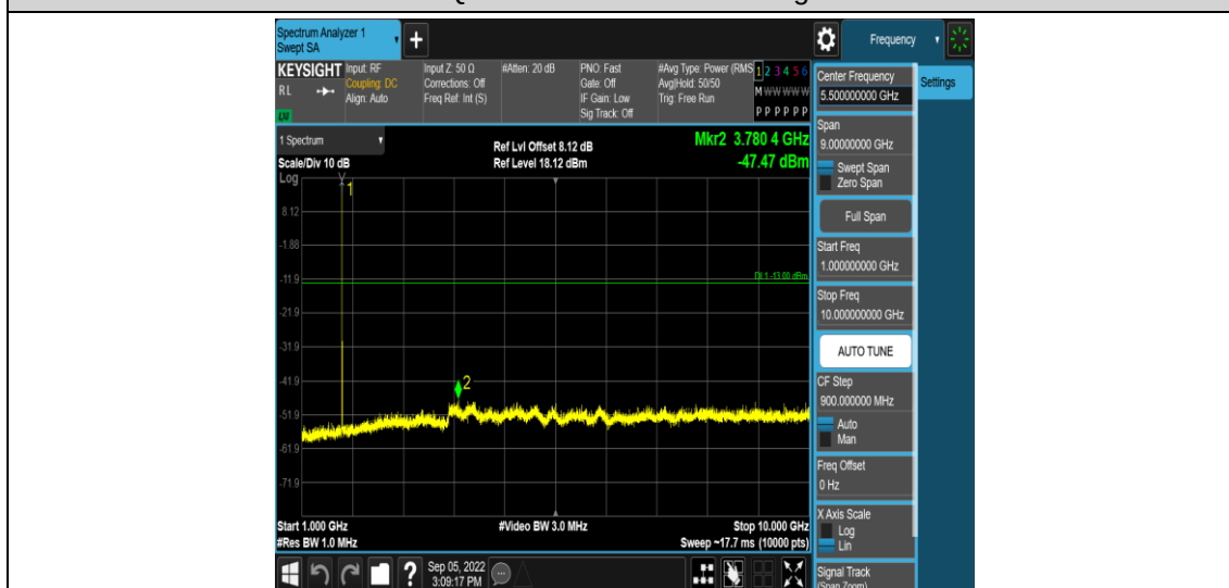
Band66-1.4MHz-QPSK-131979-1RB#0-Range4:1000~10000MHz
