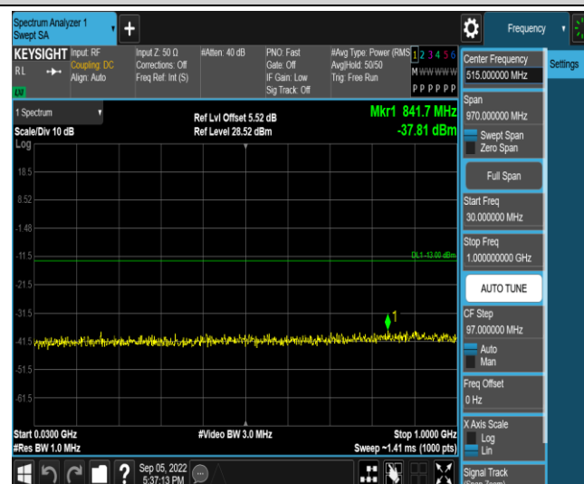
Band66-20MHz-QPSK-132322-1RB#0-Range3:30~1000MHz
