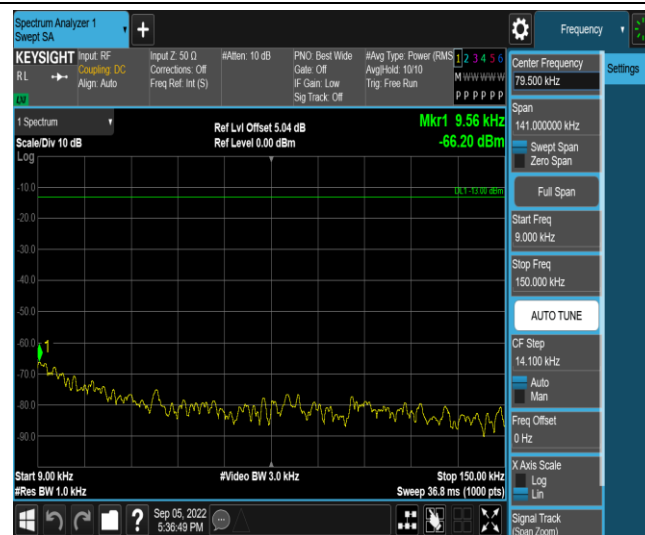
Band66-20MHz-QPSK-132322-1RB#0-Range1:0.009~0.15MHz
