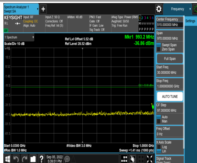
Band66-20MHz-16QAM-132572-1RB#0-Range3:30~1000MHz
