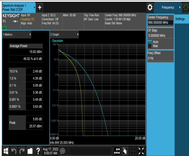
Band71-15MHz-QPSK-133397-75RB#0
