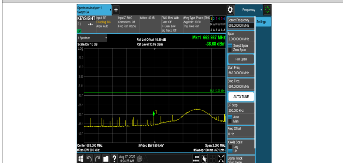
Band71-10MHz-16QAM-133172-1RB#49
