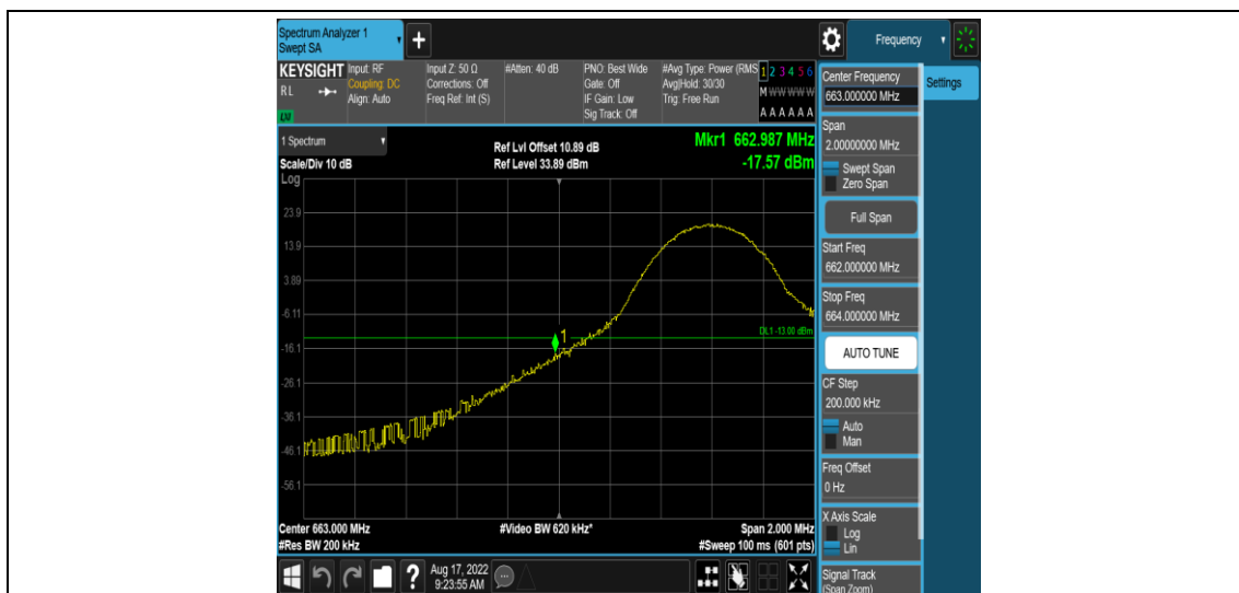
Band71-10MHz-16QAM-133172-1RB#0
