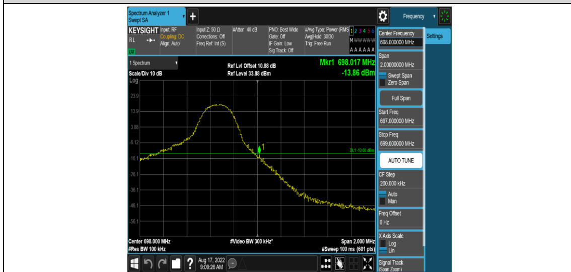
Band71-5MHz-16QAM-133447-1RB#24
