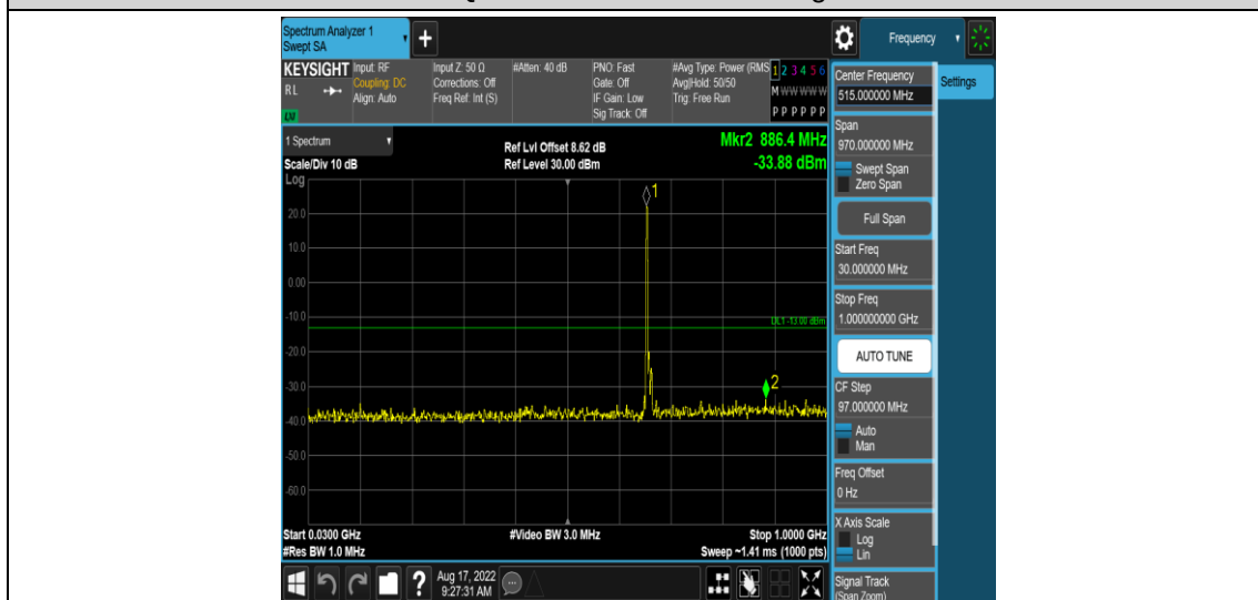
Band71-10MHz-QPSK-133172-1RB#0-Range3:30~1000MHz
