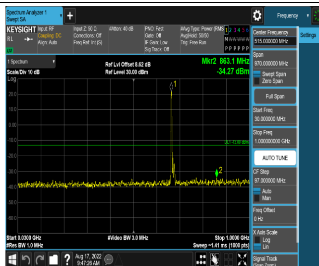
Band71-15MHz-QPSK-133297-1RB#0-Range3:30~1000MHz
