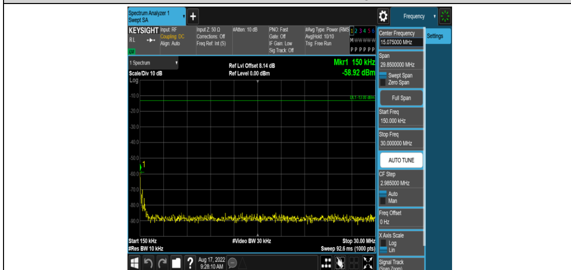
Band71-10MHz-16QAM-133172-1RB#0-Range2:0.15~30MHz
