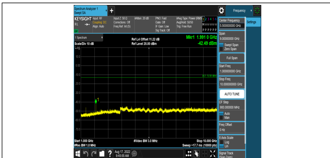
Band71-15MHz-QPSK-133197-1RB#0-Range4:1000~10000MHz
