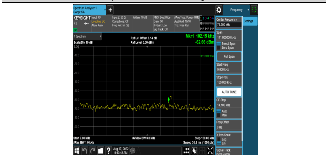
Band71-5MHz-QPSK-133447-1RB#0-Range1:0.009~0.15MHz
