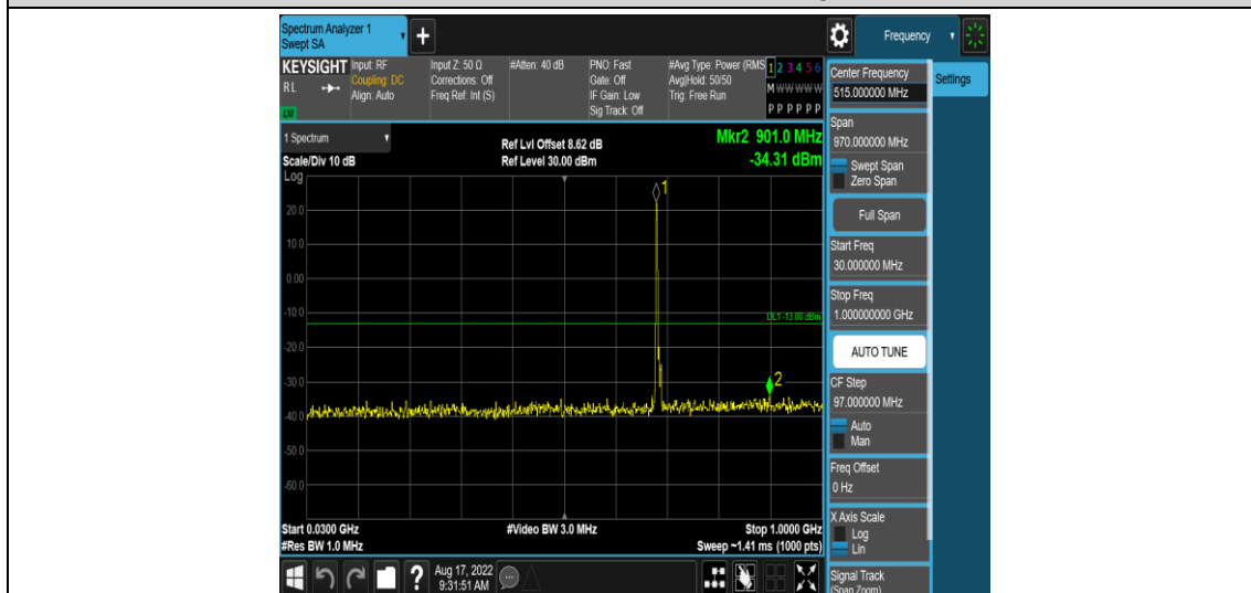
Band71-10MHz-16QAM-133422-1RB#0-Range3:30~1000MHz
