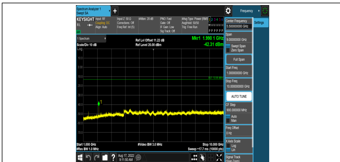
Band71-5MHz-16QAM-133147-1RB#0-Range4:1000~10000MHz
