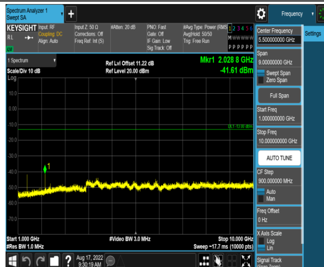
Band71-10MHz-16QAM-133297-1RB#0-Range4:1000~10000MHz
