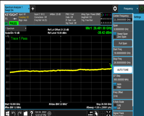
1-N41-PC3-30-100-M-4-N/A-DFT-QPSK-Edge_1RB_Left-1@0-18000-26500-Ant1-26481. 30--38.42--25-PASS
