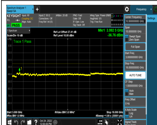
1-N41-PC3-30-100-M-4-N/A-DFT-QPSK-Edge_1RB_Left-1@0-3000-18000-Ant1-3992.50- -36.76--25-PASS
