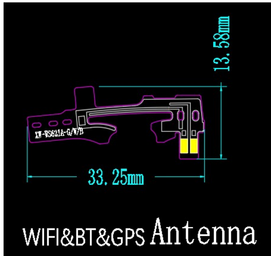
Dimensional drawing of diversity antenna
