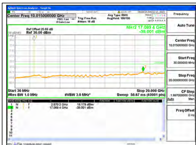
B38-30M-20G / 5MHz / Low CH / QPSK
