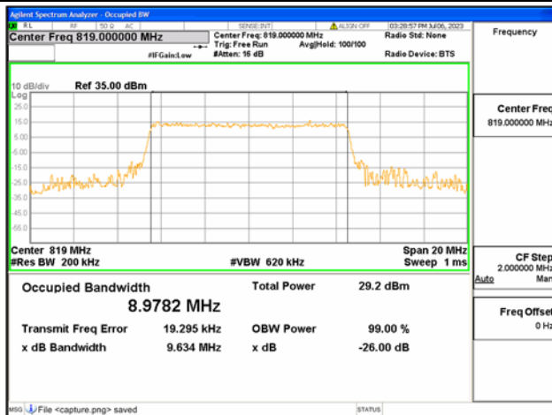
Band26 Part90 / 10MHz / 16QAM/ High CH
