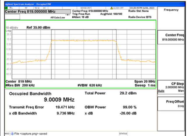
Band26 Part90 / 10MHz / QPSK/ High CH
