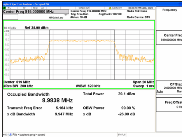
Band26 Part90 / 10MHz / 64QAM/ Mid CH
