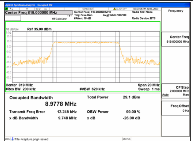
Band26 Part90 / 10MHz / 64QAM/ High CH
