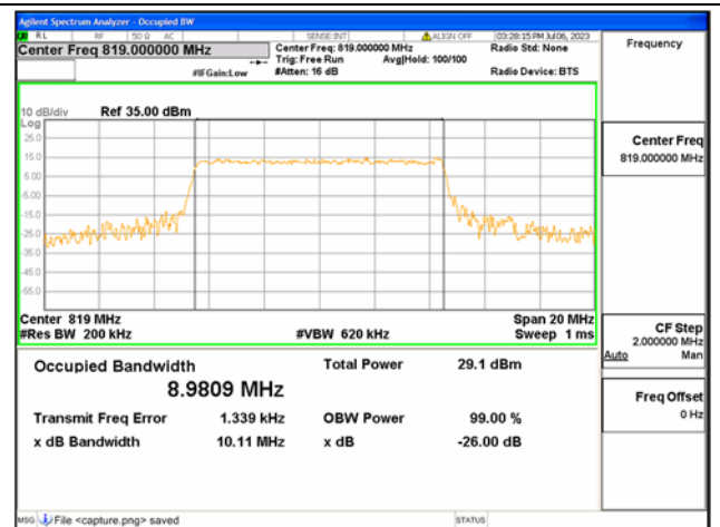
Band26 Part90 / 10MHz / 64QAM/ Low CH
