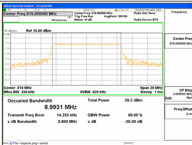
Band26 Part90 / 10MHz / 16QAM/ Low CH
