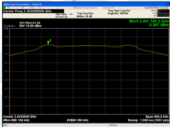
Spurious LE_Channel 0
