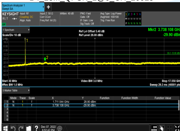
B4 15M QPSK 1@0 CH 20025
