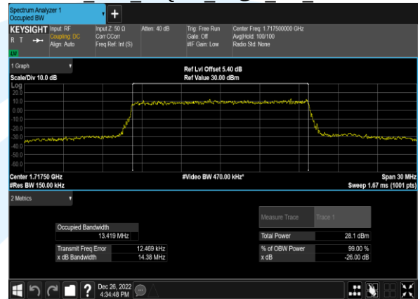
B4 15M 64QAM 75@0 CH 20325
