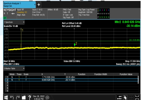
B4 1.4M 64QAM 1@0 CH 19957
