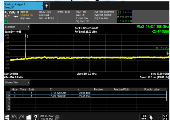
B4 10M 16QAM 1@0 CH 20175
