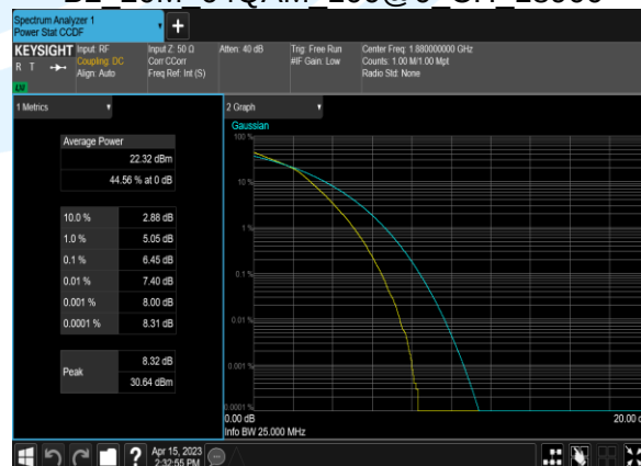
B2 20M 64QAM 100@0 CH 18900
