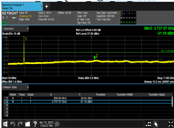
B12 10M QPSK 1@0 CH 23060
