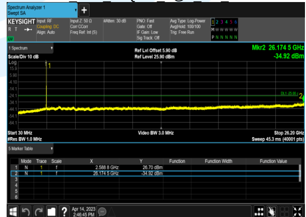
B38 15M 16QAM 1@0 CH 38000
