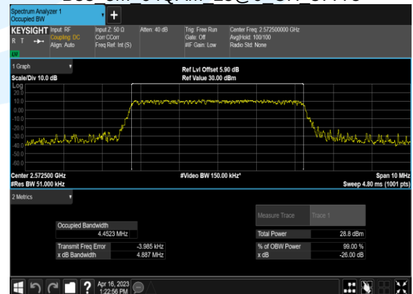
B38 5M 64QAM 25@0 CH 37775
