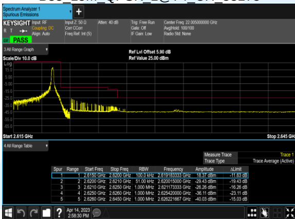
B38 15M 16QAM 1@74 CH 38175
