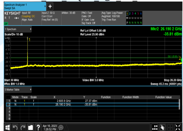
B38 10M 64QAM 1@0 CH 38000
