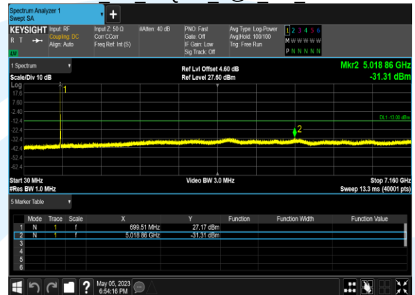
B12 5M 64QAM 1@0 CH 23155
