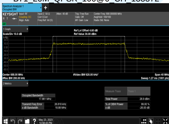
B71_20M_QPSK_100@0_CH_133372
