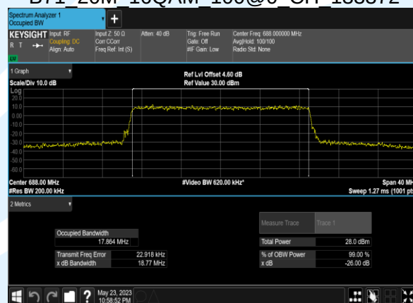
B71_20M_16QAM_100@0_CH_133372
