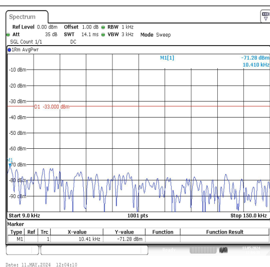
Band26_15MHz_16QAM_26915_1RB#0_0.009~0.15_0.009~0.15
