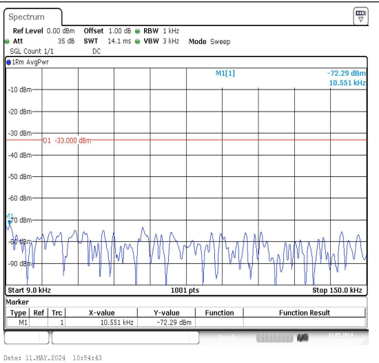
Band26_5MHz_16QAM_26815_1RB#0_0.009~0.15_0.009~0.15
