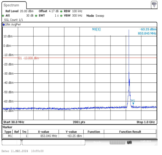
Band26_5MHz_16QAM_26815_1RB#0_30~1000_30~1000
