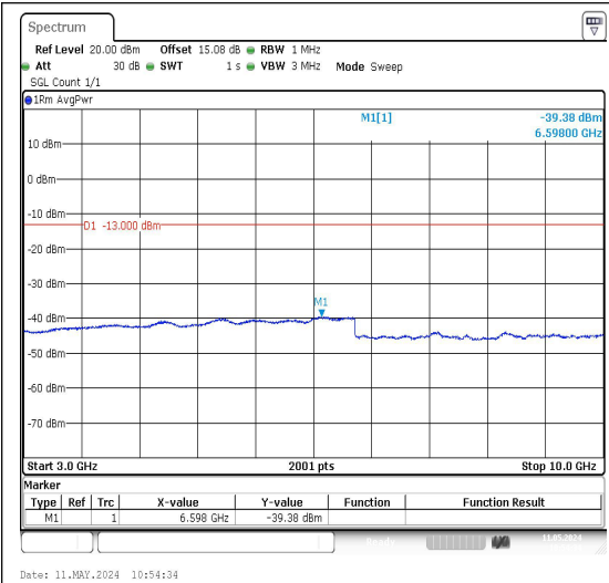
Band26_5MHz_QPSK_26815_1RB#0_3000~10000_3000~10000
