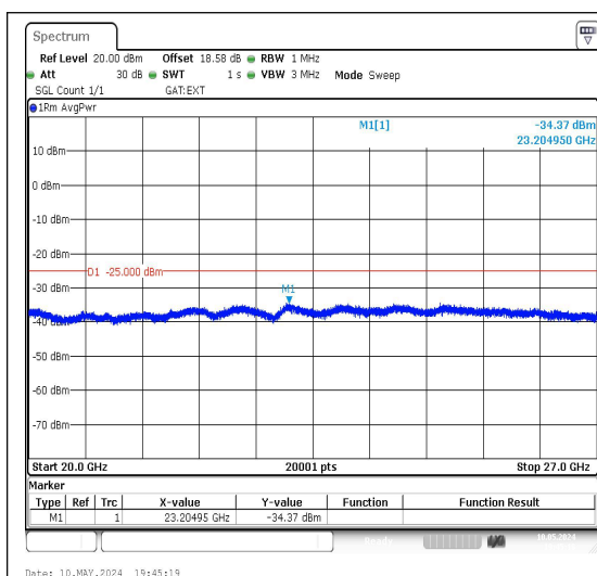
Band38_20MHz_QPSK_37850_1RB#0_20000~27000
