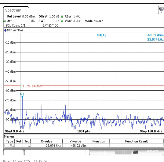
Band38_20MHz_16QAM_37850_1RB#0_0.009~0.15
