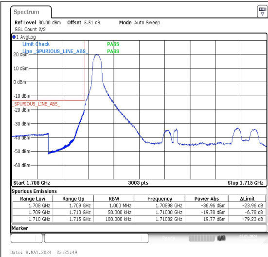
Band4_5MHz_QPSK_19975_1RB#0
