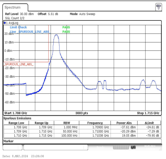
Band4_5MHz_16QAM_19975_1RB#0
