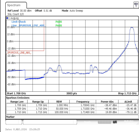
Band4_5MHz_QPSK_19975_1RB#24
