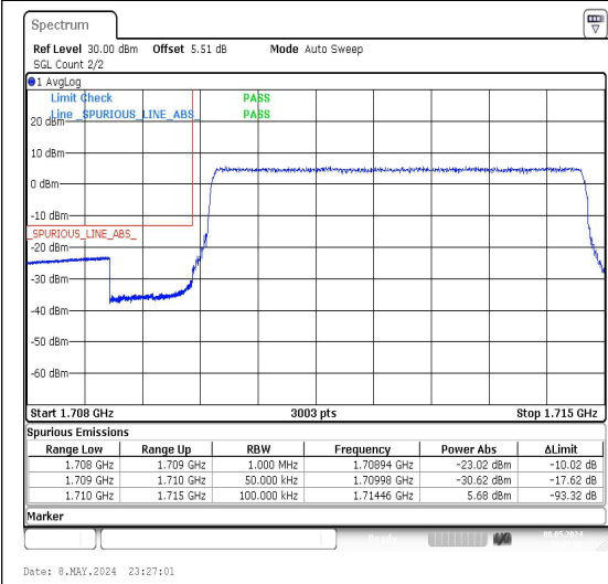
Band4_5MHz_QPSK_19975_25RB#0
