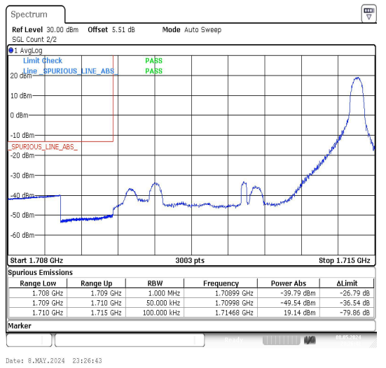
Band4_5MHz_16QAM_19975_1RB#24
