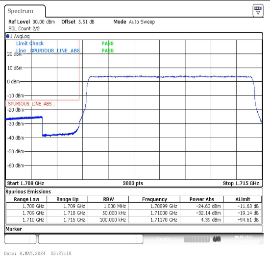
Band4_5MHz_16QAM_19975_25RB#0
