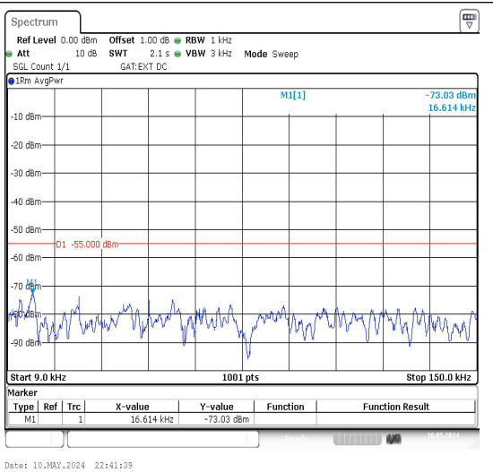
Band41_15MHz_16QAM_41515_1RB#0_0.009~0.15_0.009~0.15
