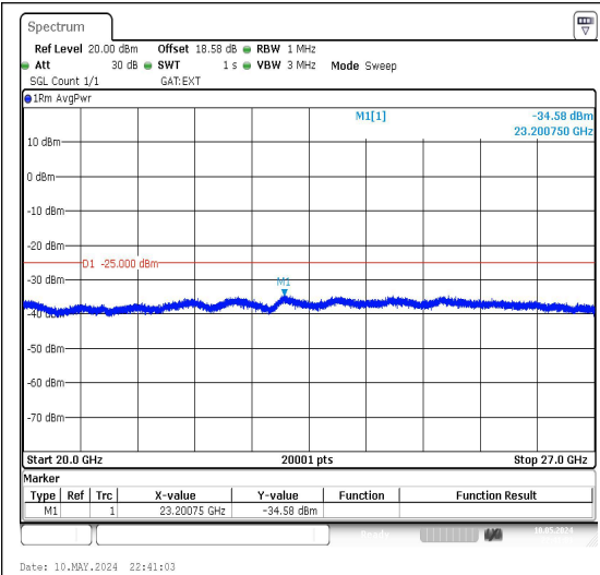
Band41_15MHz_QPSK_41515_1RB#0_20000~27000_20000~27000
