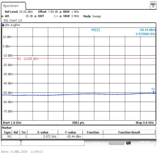
Band71_20MHz_QPSK_133372_1RB#0_1000~3000_00_1000~3000
