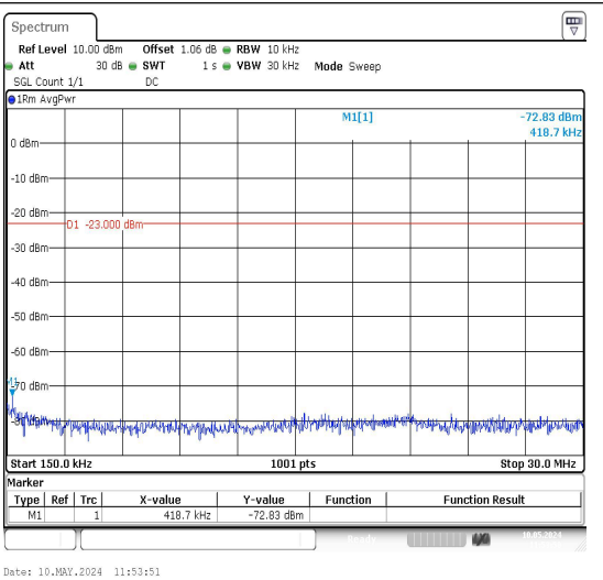
Band71_20MHz_QPSK_133372_1RB#0_0.15~30_0.15~30
