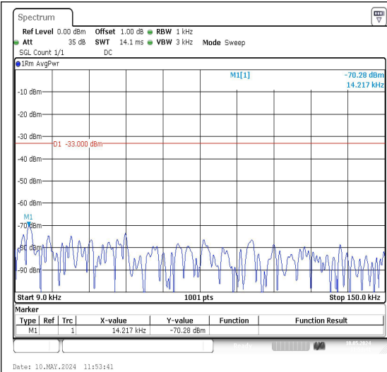
Band71_20MHz_QPSK_133372_1RB#0_0.009~0.15_0.009~0.15
