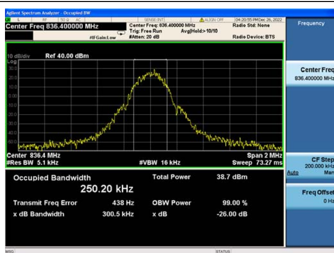
GSM850(GSM), CH189, 836.4MHz
