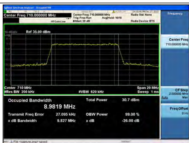
Band17 / 10MHz / 16QAM/ Mid CH
