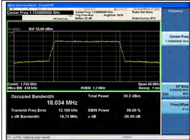
Band66 / 20MHz / 64QAM/ Mid CH
