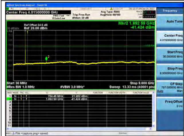
Band17 / 5MHz / Low CH / 64QAM
