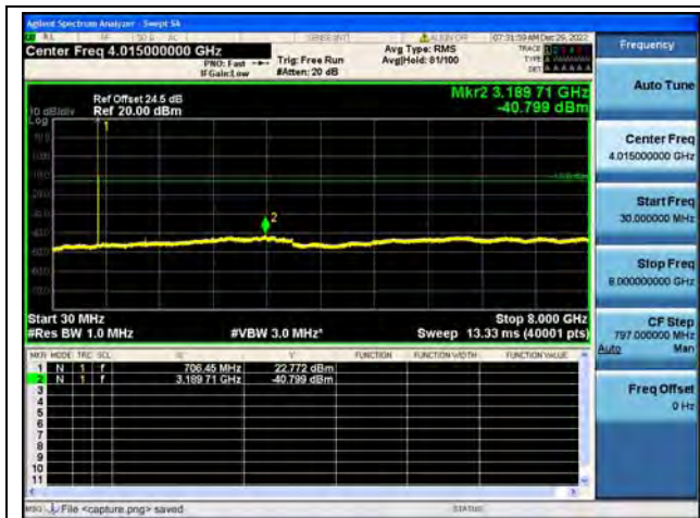
Band12 / 3MHz / Mid CH / QPSK
