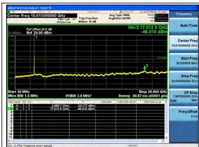
Band7-30M-20G / 20MHz / High CH / QPSK
