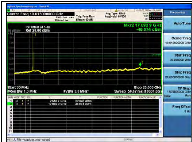
Band7-30M-20G / 15MHz / High CH / QPSK
