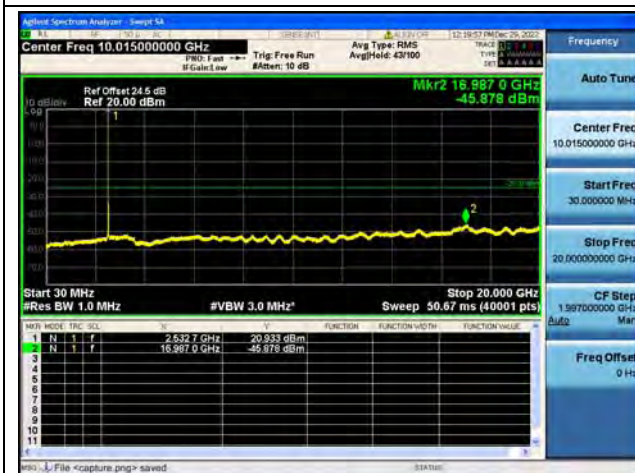
Band7-30M-20G / 5MHz / Mid CH / 64QAM
