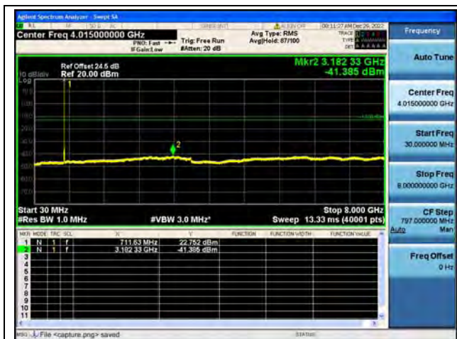
Band17 / 5MHz / High CH / QPSK
