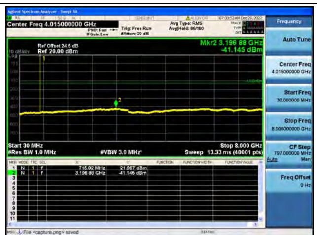
Band12 / 1.4MHz / High CH / 16QAM
