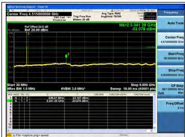
Band5 / 3MHz / Mid CH / QPSK
