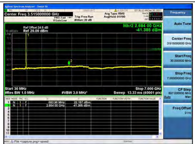
Band71 / 15MHz / High CH / 16QAM
