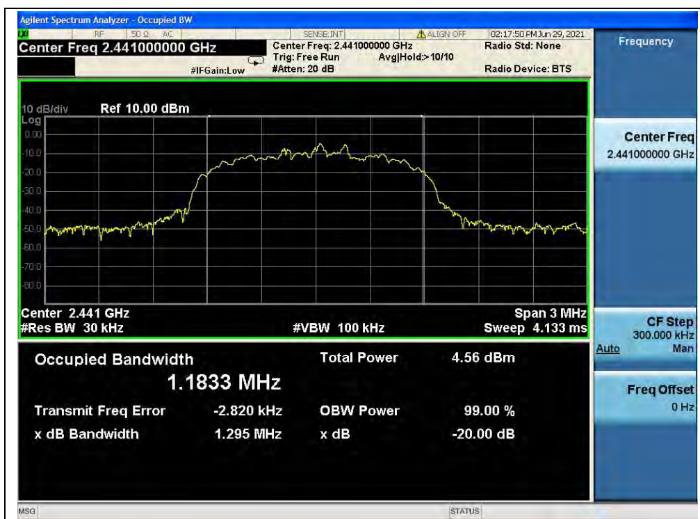
(Channel 39, 8-DPSK)
