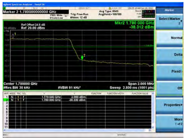
Band66 / 1.4MHz / High CH / QPSK / FULL RB
