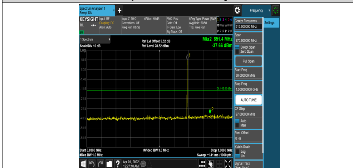
Band12-5MHz-QPSK-23035-1RB#0-Range3:30~1000MHz
