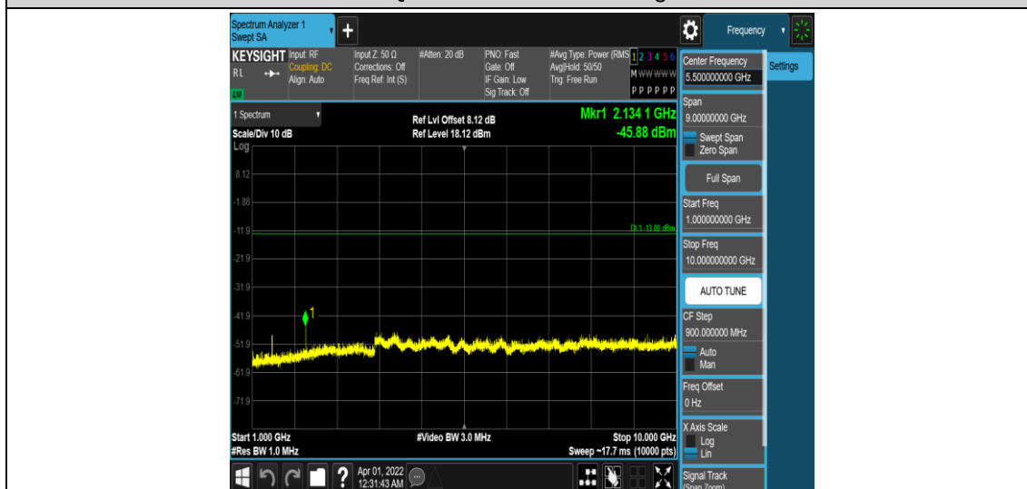
Band12-5MHz-16QAM-23155-1RB#0-Range4:1000~10000MHz
