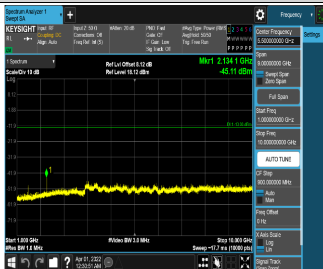
Band12-5MHz-QPSK-23155-1RB#0-Range4:1000~10000MHz
