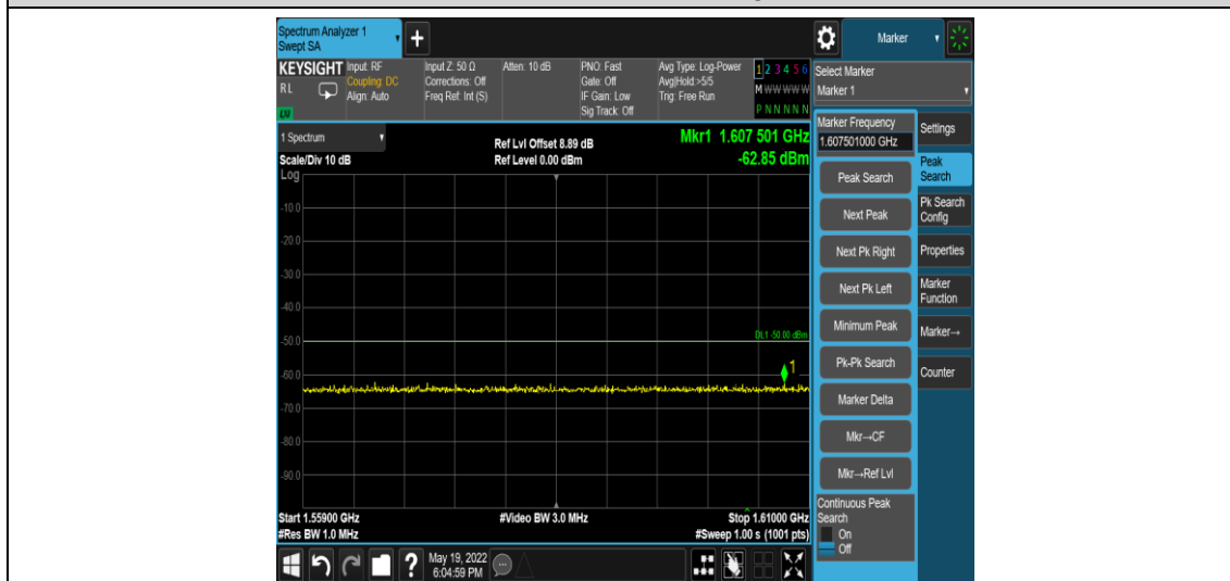
Band13-5MHz-QPSK-23255-1RB#0-Range7:1559~1610MHz
