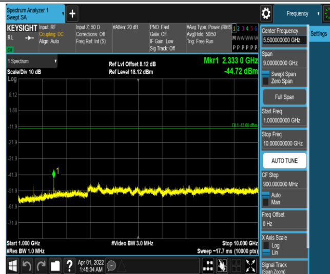
Band13-10MHz-QPSK-23230-1RB#0-Range4:1000~10000MHz
