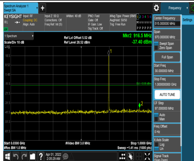
Band17-5MHz-QPSK-23755-1RB#0-Range3:30~1000MHz
