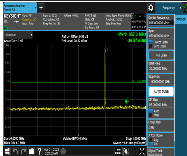
Band17-10MHz-16QAM-23780-1RB#0-Range3:30~1000MHz
