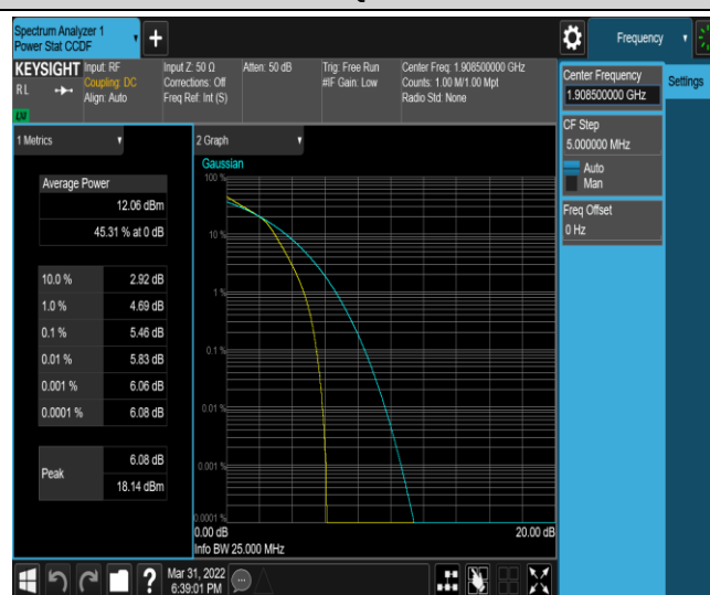
Band2-3MHz-16QAM-19185-15RB#0
