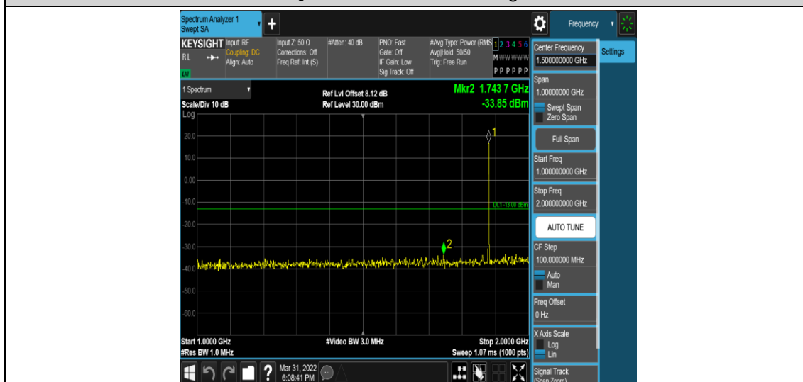
Band2-1.4MHz-QPSK-18900-1RB#0-Range4:1000~2000MHz
