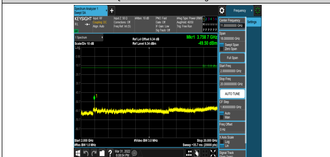
Band2-1.4MHz-QPSK-18900-1RB#0-Range5:2000~20000MHz
