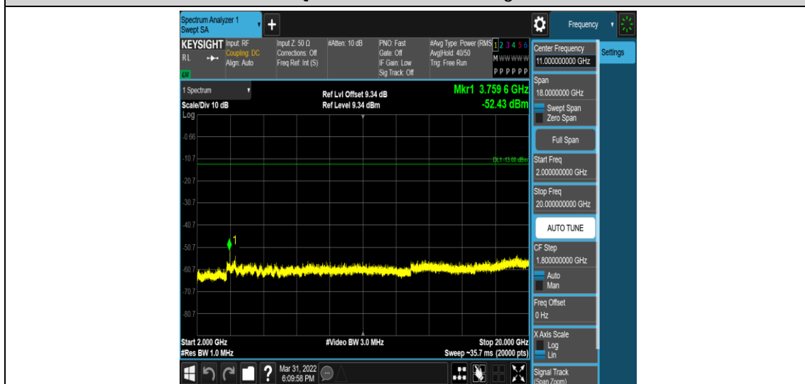
Band2-1.4MHz-16QAM-18900-1RB#0-Range5:2000~20000MHz
