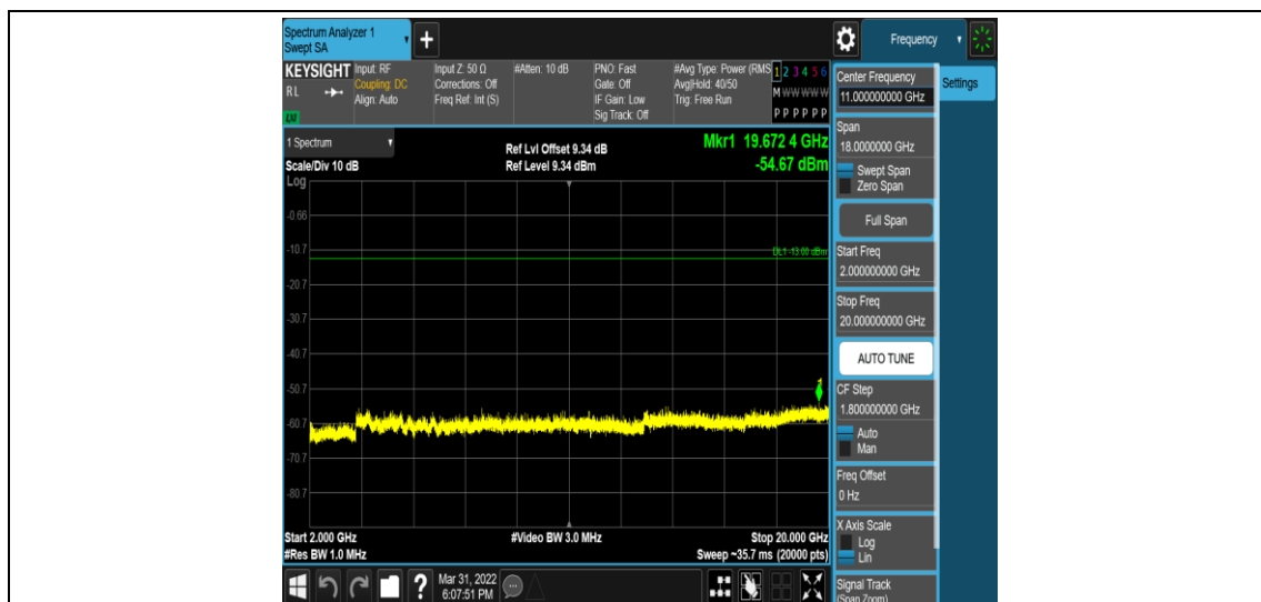
Band2-1.4MHz-16QAM-18607-1RB#0-Range5:2000~20000MHz
