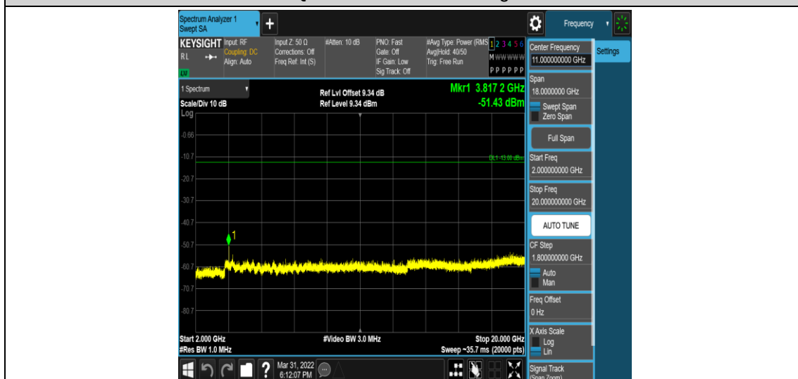
Band2-1.4MHz-16QAM-19193-1RB#0-Range5:2000~20000MHz
