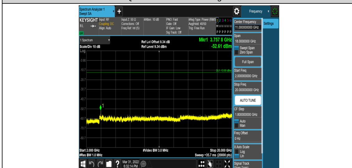
Band2-3MHz-16QAM-18900-1RB#0-Range5:2000~20000MHz
