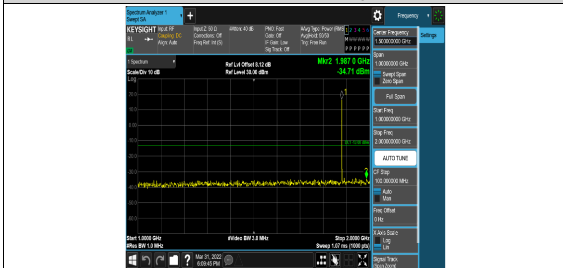
Band2-1.4MHz-16QAM-18900-1RB#0-Range4:1000~2000MHz
