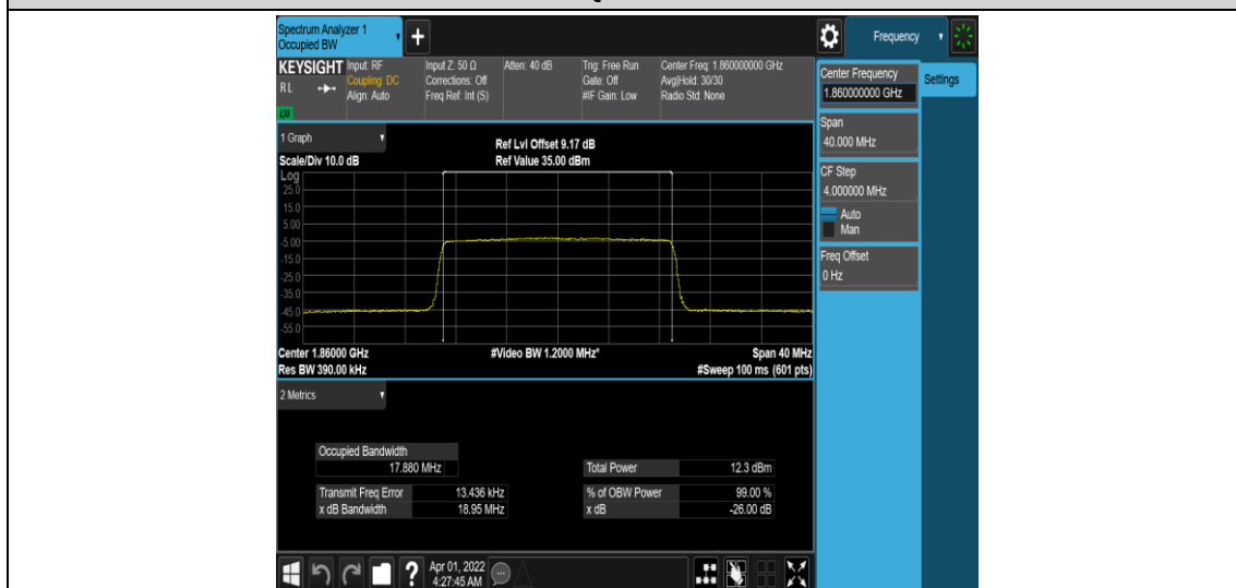
Band25-20MHz-16QAM-26140-100RB#0
