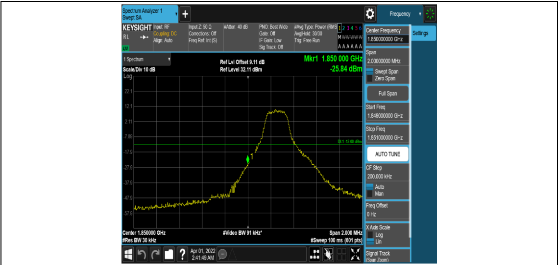
Band25-1.4MHz-QPSK-26047-1RB#0
