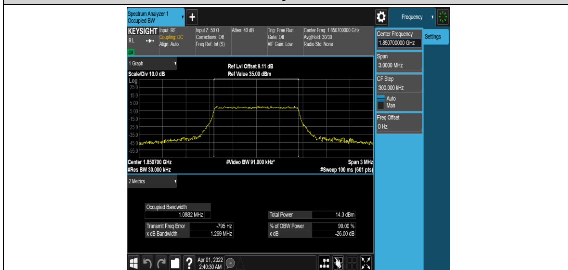
Band25-1.4MHz-16QAM-26047-6RB#0
