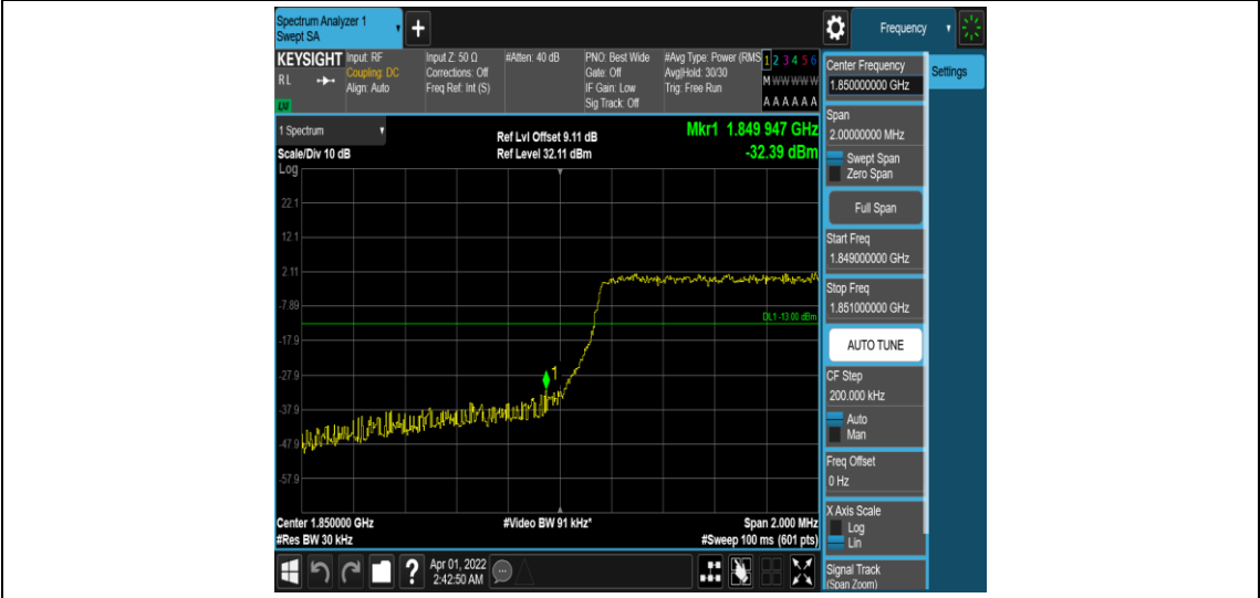
Band25-1.4MHz-QPSK-26047-6RB#0
