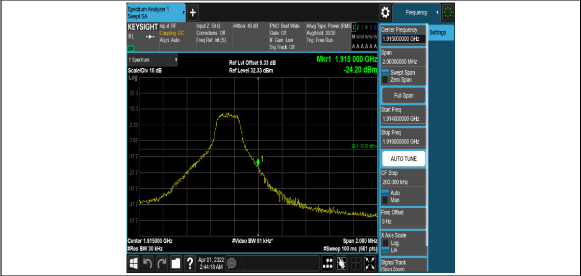
Band25-1.4MHz-16QAM-26683-1RB#5
