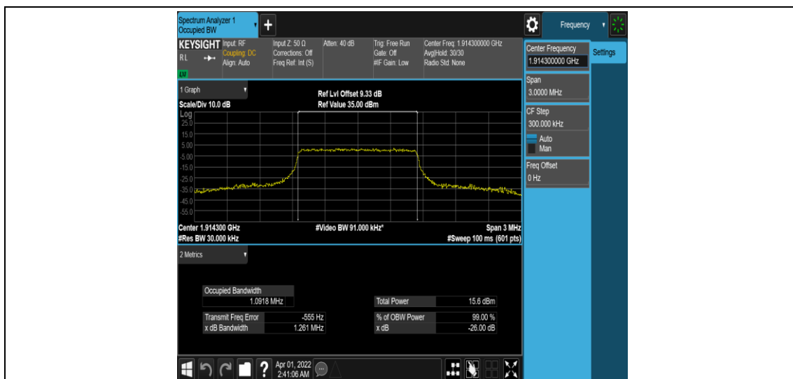
Band25-1.4MHz-QPSK-26683-6RB#0
