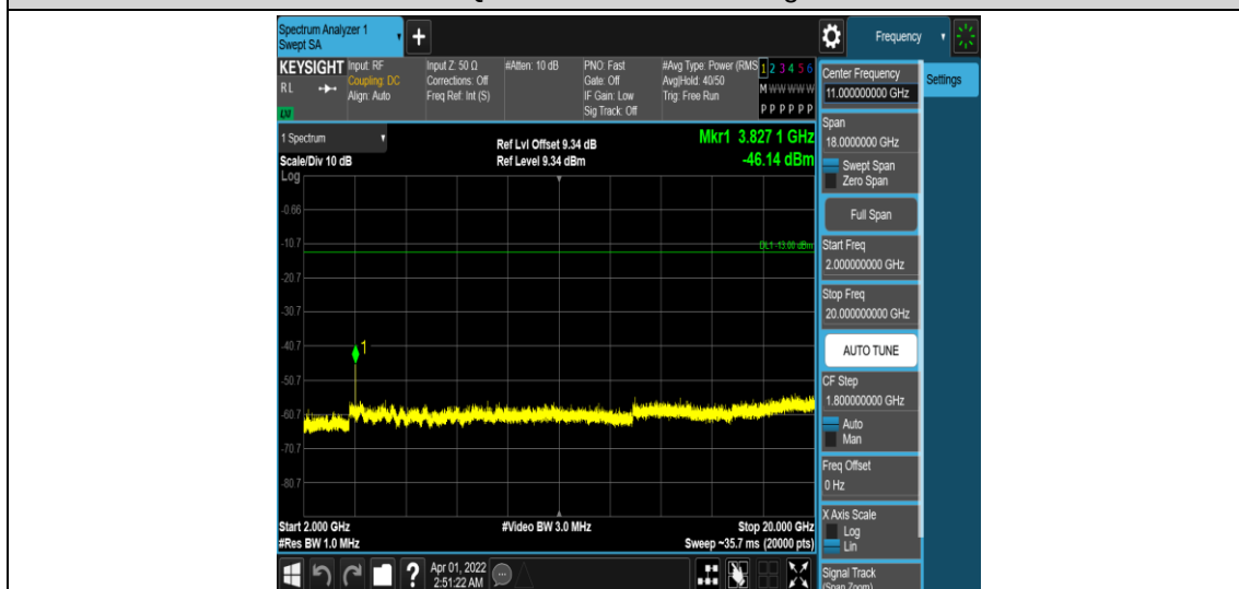
Band25-1.4MHz-16QAM-26683-1RB#0-Range5:2000~20000MHz
