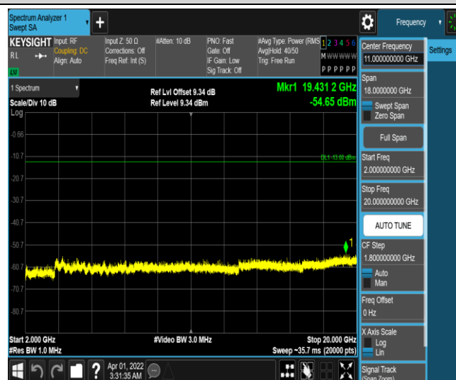
Band25-5MHz-QPSK-26365-1RB#0-Range5:2000~20000MHz
