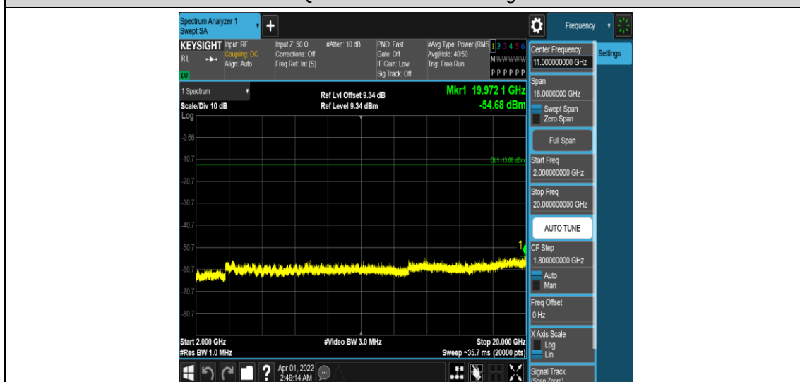
Band25-1.4MHz-16QAM-26365-1RB#0-Range5:2000~20000MHz
