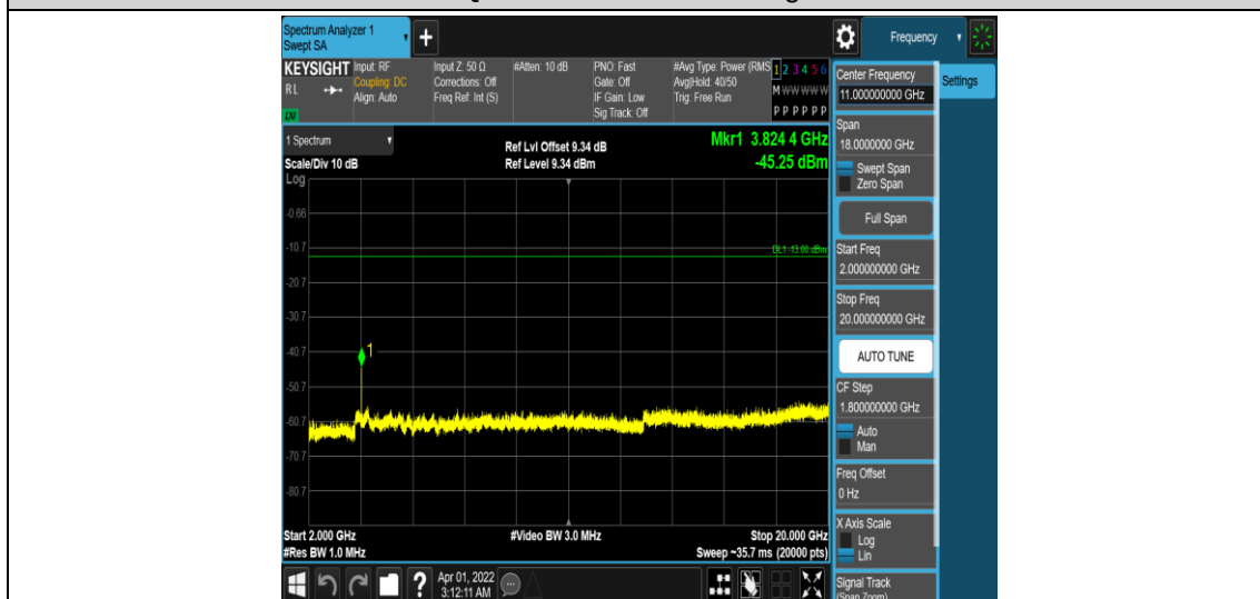
Band25-3MHz-16QAM-26675-1RB#0-Range5:2000~20000MHz
