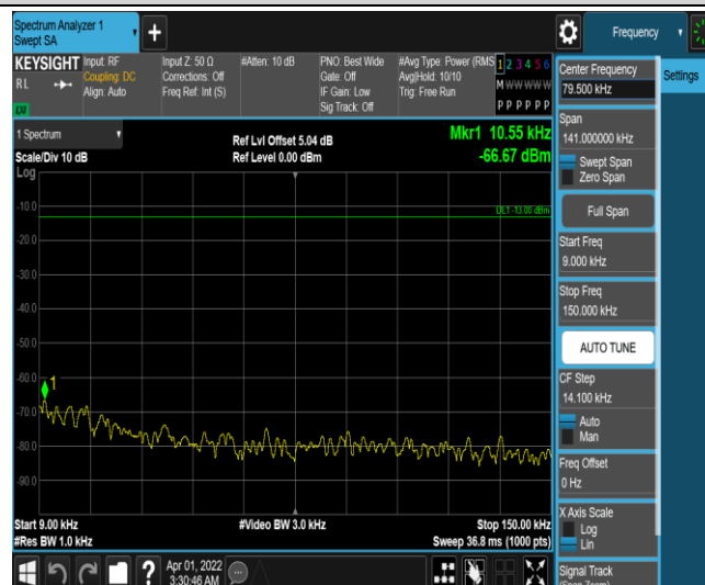
Band25-5MHz-QPSK-26365-1RB#0-Range1:0.009~0.15MHz
