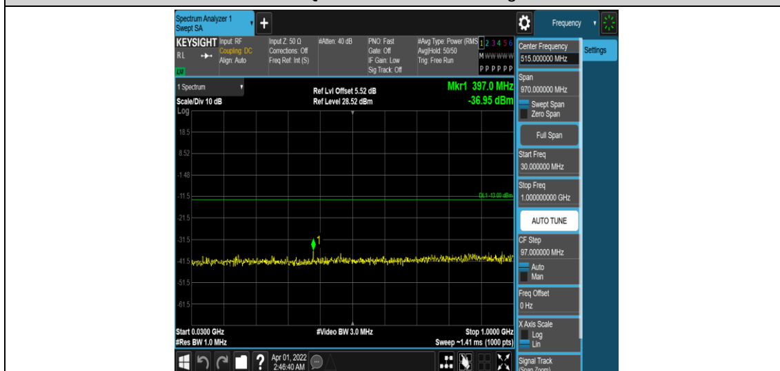
Band25-1.4MHz-16QAM-26047-1RB#0-Range3:30~1000MHz
