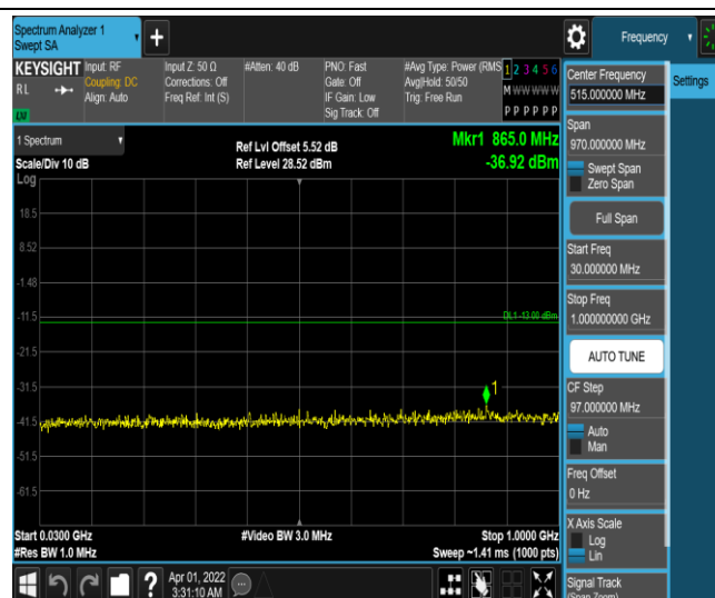
Band25-5MHz-QPSK-26365-1RB#0-Range3:30~1000MHz
