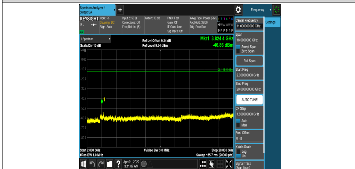
Band25-3MHz-QPSK-26675-1RB#0-Range5:2000~20000MHz
