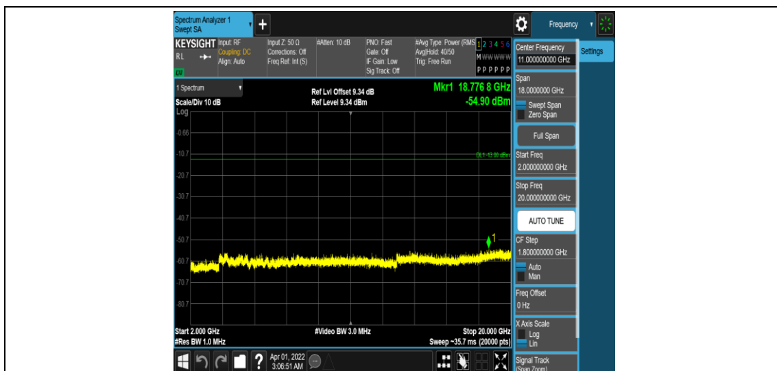
Band25-3MHz-QPSK-26055-1RB#0-Range5:2000~20000MHz
