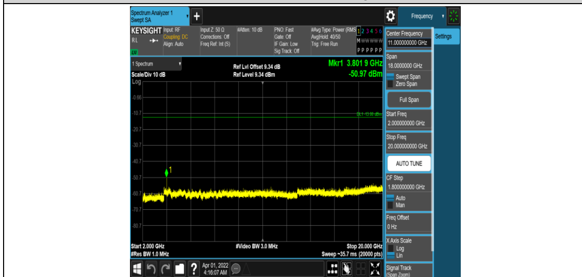
Band25-15MHz-QPSK-26615-1RB#0-Range5:2000~20000MHz
