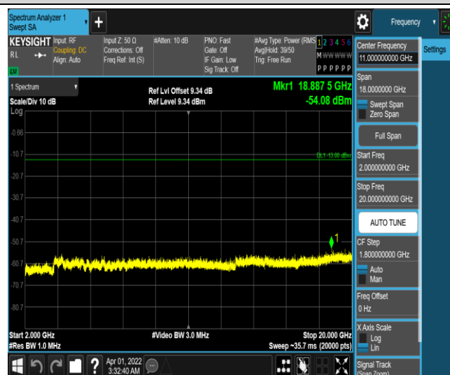
Band25-5MHz-16QAM-26365-1RB#0-Range5:2000~20000MHz
