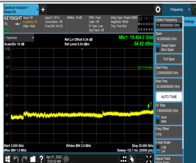
Band25-10MHz-16QAM-26365-1RB#0-Range5:2000~20000MHz
