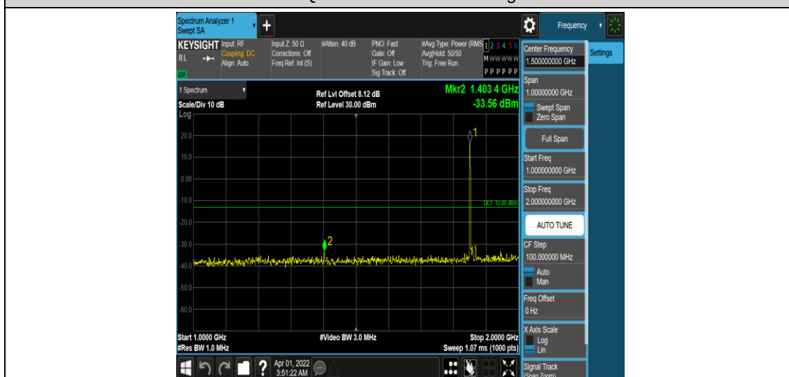
Band25-10MHz-16QAM-26090-1RB#0-Range4:1000~2000MHz
