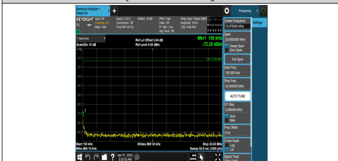
Band25-5MHz-16QAM-26365-1RB#0-Range2:0.15~30MHz
