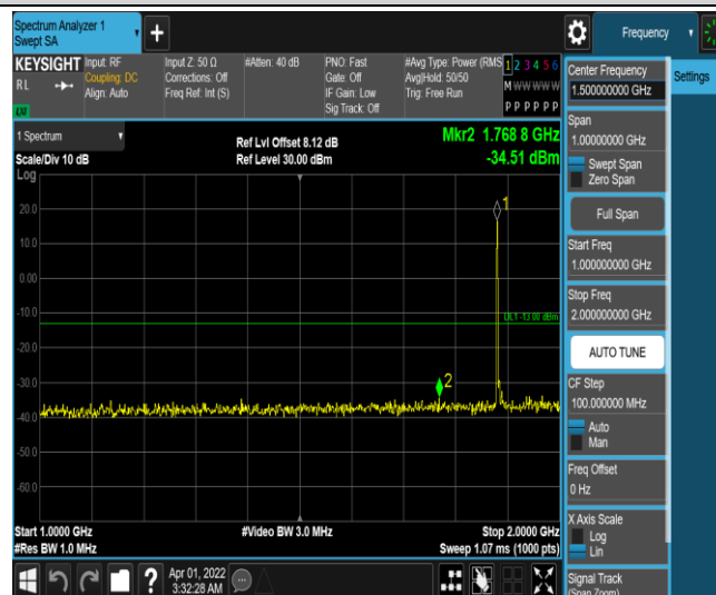
Band25-5MHz-16QAM-26365-1RB#0-Range4:1000~2000MHz
