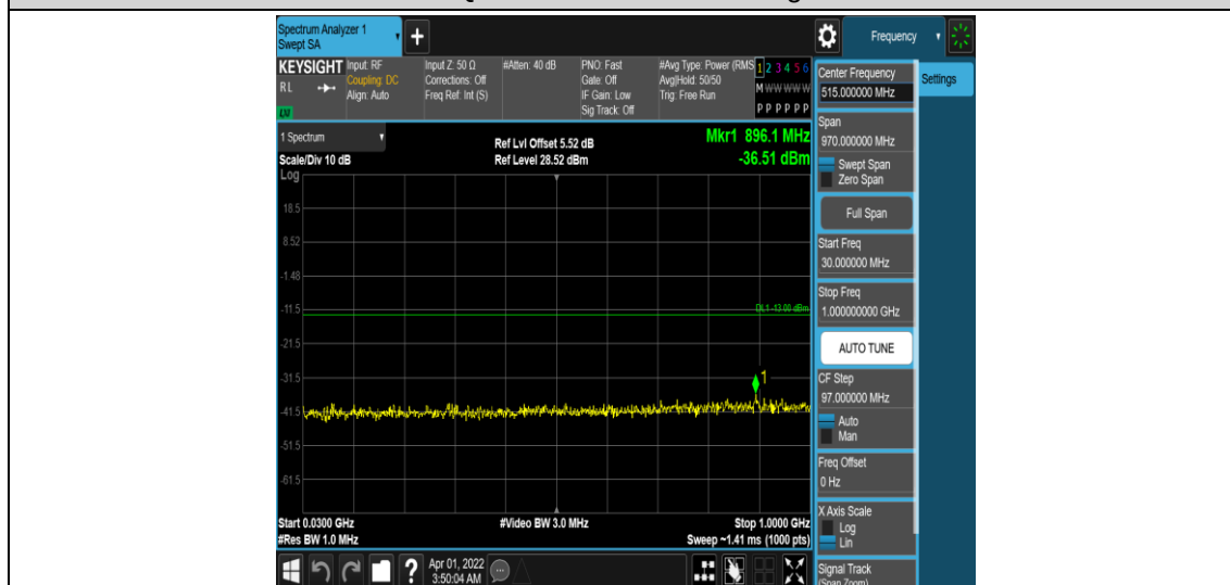
Band25-10MHz-QPSK-26090-1RB#0-Range3:30~1000MHz
