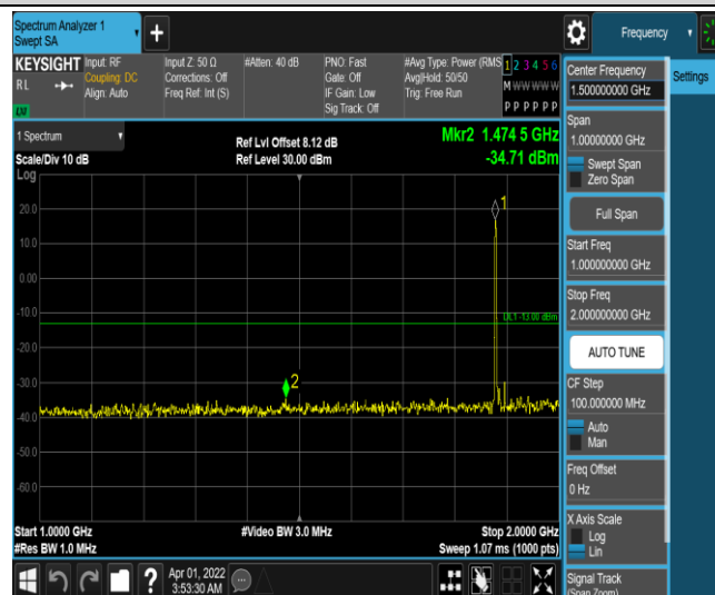
Band25-10MHz-16QAM-26365-1RB#0-Range4:1000~2000MHz
