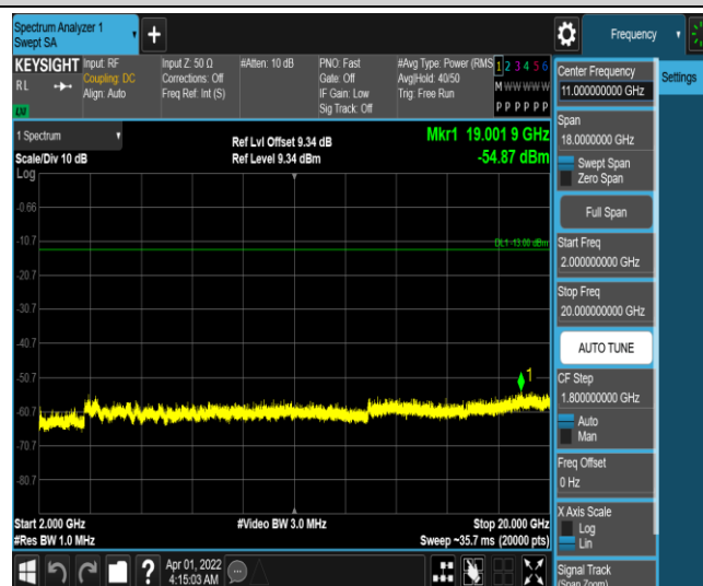
Band25-15MHz-16QAM-26365-1RB#0-Range5:2000~20000MHz
