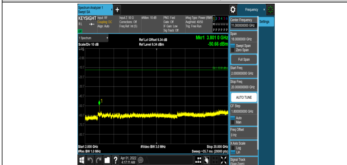
Band25-15MHz-16QAM-26615-1RB#0-Range5:2000~20000MHz
