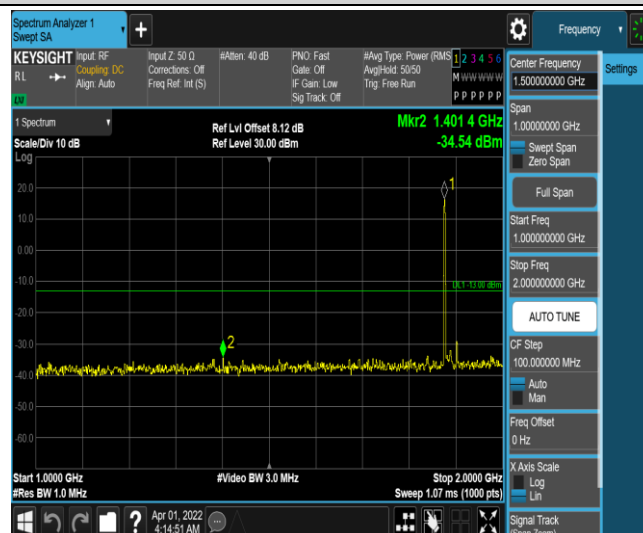
Band25-15MHz-16QAM-26365-1RB#0-Range4:1000~2000MHz
