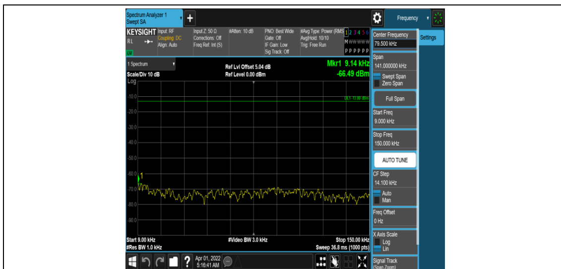
Band26-3MHz-QPSK-26775-1RB#0-Range1:0.009~0.15MHz
