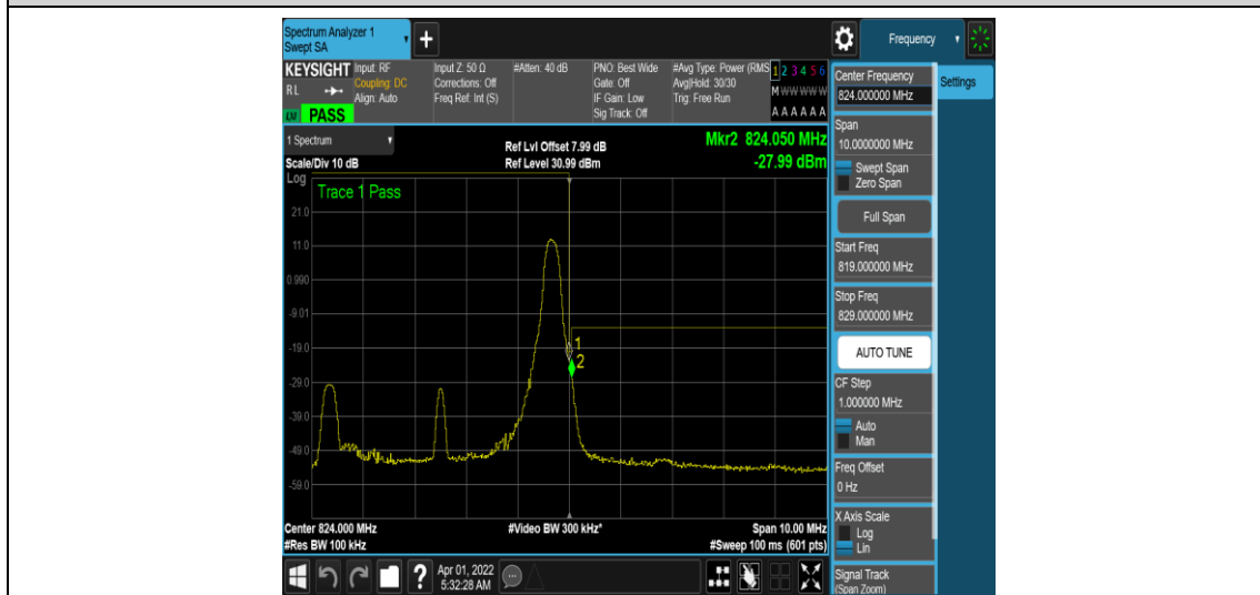
Band26-5MHz-QPSK-26765-1RB#24
