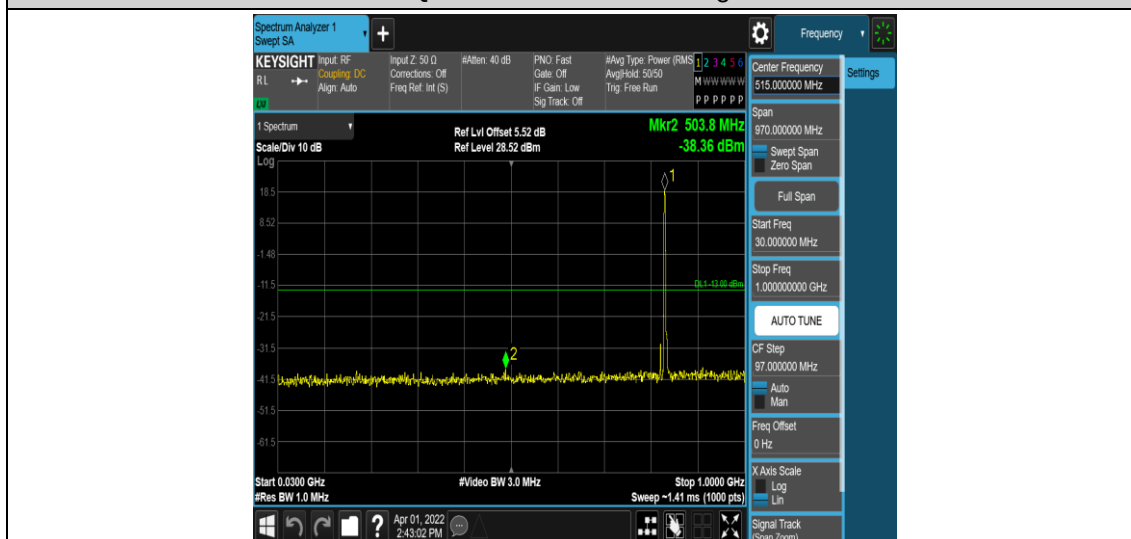
Band26-5MHz-QPSK-26915-1RB#0-Range3:30~1000MHz
