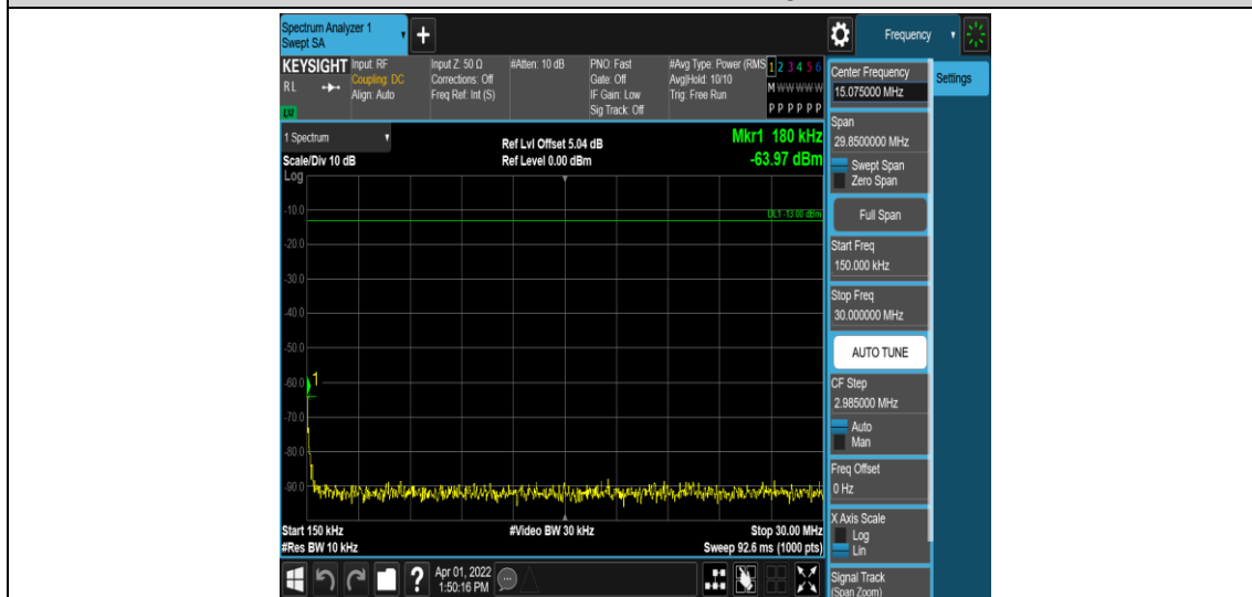
Band26-1.4MHz-QPSK-27033-1RB#0-Range2:0.15~30MHz
