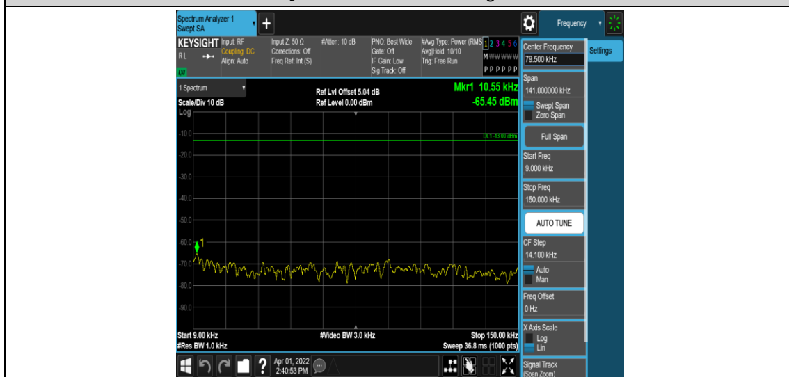
Band26-5MHz-QPSK-26815-1RB#0-Range1:0.009~0.15MHz
