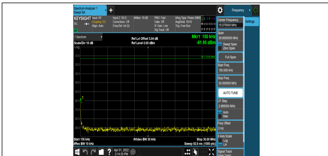
Band26-3MHz-16QAM-26915-1RB#0-Range2:0.15~30MHz
