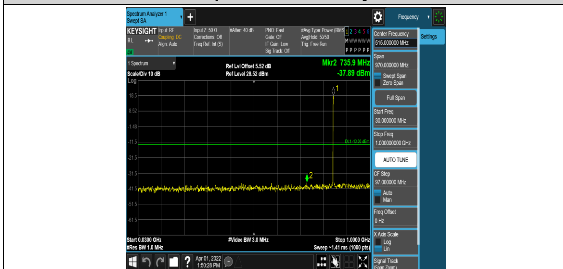
Band26-1.4MHz-QPSK-27033-1RB#0-Range3:30~1000MHz
