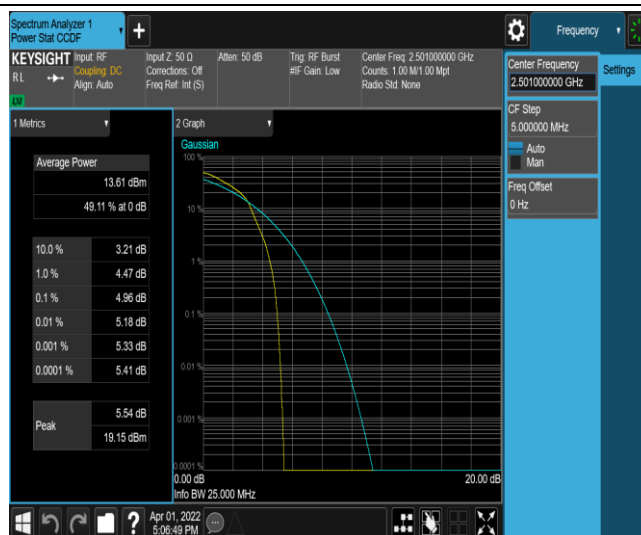
Band41-10MHz-16QAM-39700-1RB#0
