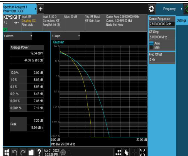
Band41-15MHz-16QAM-40620-75RB#0
