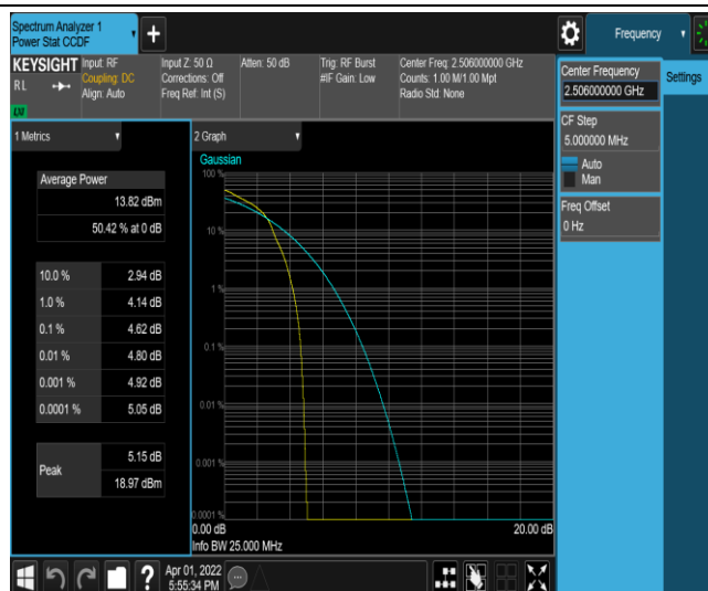
Band41-20MHz-16QAM-39750-1RB#0
