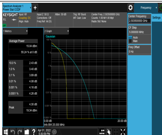
Band41-15MHz-QPSK-39725-1RB#0
