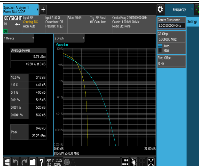
Band41-15MHz-16QAM-39725-1RB#0
