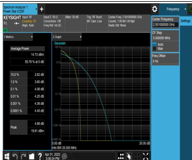
Band41-10MHz-QPSK-39700-1RB#0
