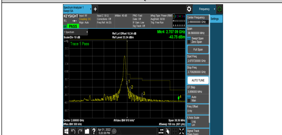
Band41-15MHz-16QAM-41515-1RB#74
