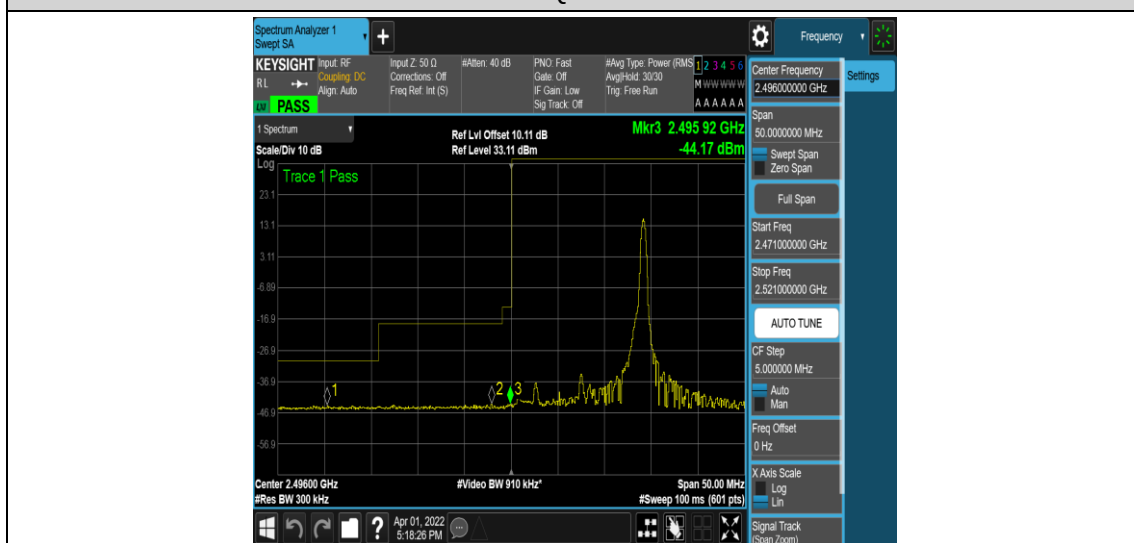
Band41-15MHz-QPSK-39725-1RB#74
