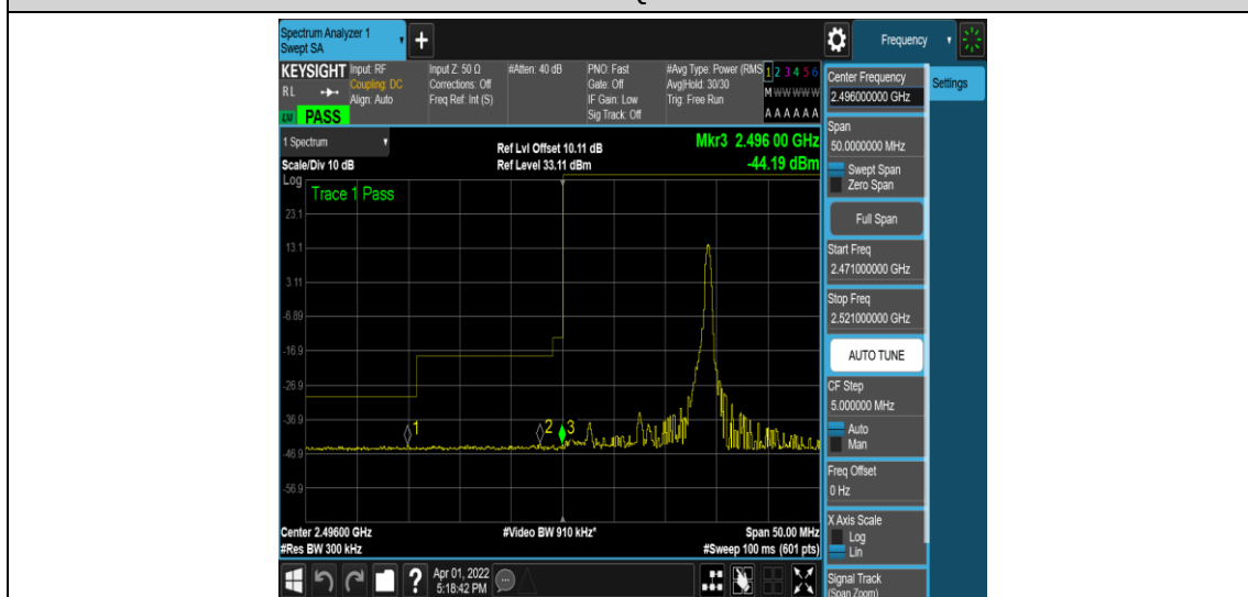
Band41-15MHz-16QAM-39725-1RB#74
